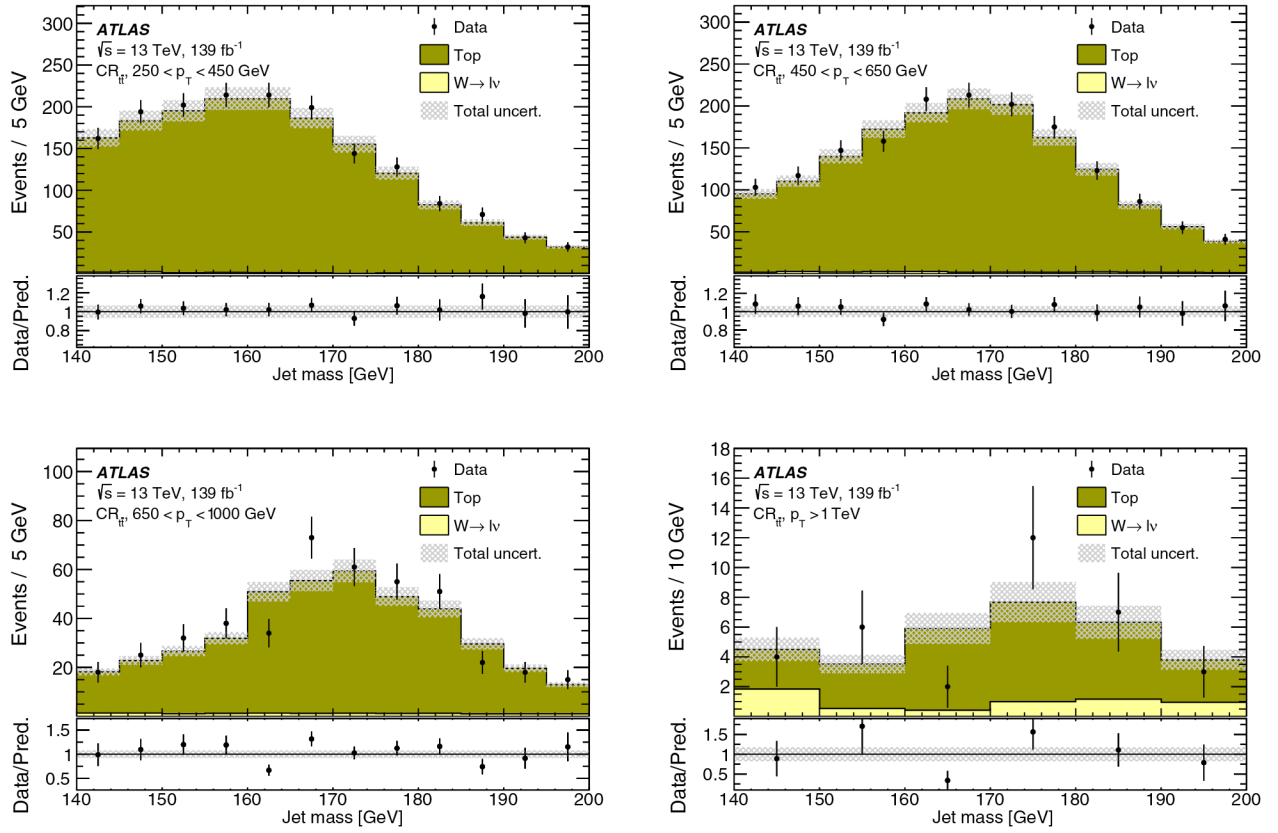
FIG. 3. The post-fit CR_{H} J_t mass distribution in the four p_T regions used in the global likelihood of the differential fit (Sec. IX C). The W(\ell\nu) contribution is flat in jet mass and for events with p_T < 1 TeV it is estimated to be 1–3% of the total. The p_T > 1 TeV region is shown in 10 GeV jet mass bins. The ratio of the data to the background prediction is shown in the lower panel. The shaded areas indicate the 68% CL for all background processes.
