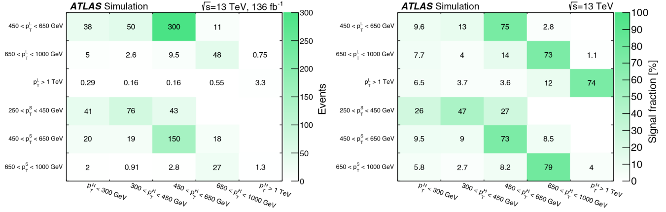
FIG. 8. For each of the p_T^H differential volumes (x-axis), the expected signal event yield for all Higgs boson events (left) and the fraction of signal in percent (right) in each reconstructed jet p_T region (y-axis) is shown. The leading jet's p_T in the SRL is denoted by p_T^L and the subleading jet's p_T in the SRS is denoted by p_T^S .
