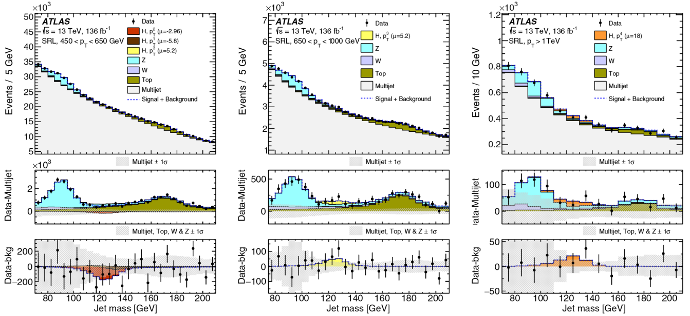
FIG. 11. Post-fit jet mass distributions of the various components in the differential leading-jet signal region defined by the selected candidate jet with 450 < p_T < 650 GeV (left), 650 < p_T < 1000 GeV (middle), and p_T > 1000 GeV (right) shown in wider 10 GeV bins. The middle panels show the distributions after subtraction of the multijet distribution. The shaded areas indicate the 68% CL for the multijet background from the fitted parameters and normalizations of the exponentiated polynomials. The lower panels show the distributions after subtraction of all the fitted background processes: multijet, V + jets, and Top. The shaded areas indicate the 68% CL for all background processes. The five STXS volumes are labeled p_T^0-p_T^4 corresponding to p_T^H < 300 GeV, 300-450 GeV, 450-650 GeV, 650-1000 GeV, and >1000 GeV, respectively. The p_T^0 event yield is constrained to its SM value within the theoretical and experimental uncertainties and free parameters act independently on the remaining four volumes. Contributions below 0.5 per mille of the total yield are not shown.
