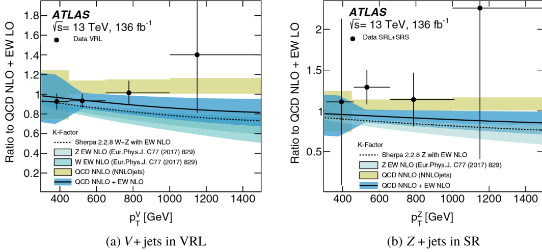
FIG. 9. Comparison of differential fit signal strengths for (a) V + jets in the VRL and (b) Z + jets in the SR. The signal strength within the STXS volumes is calculated relative to the prediction at NLO QCD and LO EW accuracy. They are compared with the NLO EW correction provided by SHERPA, the NNLO QCD correction provided by the NNLOJET group, and their product. The Higgs boson yields are kept fixed to the SM expectation when extracting the Z + jets signal strength within the STXS volumes. The points are located at the weighted center of the bin considering the underlying p_T^V or p_T^H spectrum.
