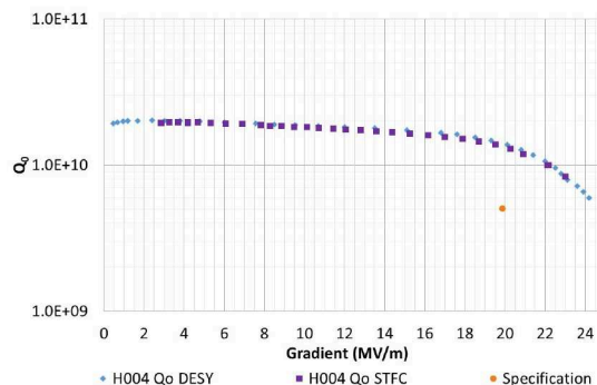
Figure 4: H004 cavity test results at DESY and STFC.
