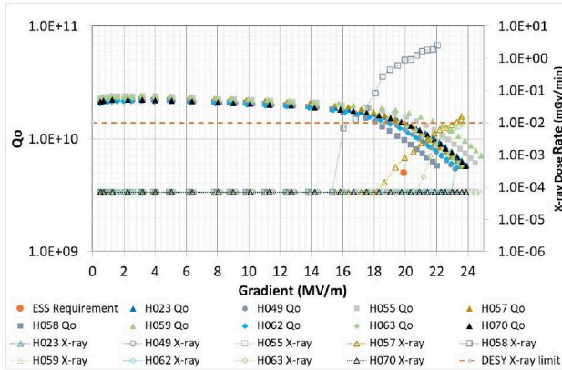
Figure 6: Production testing of cavities at DESY with a 24-hour HPR.
