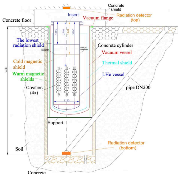
Figure 2: Schematic of DESY test system.
