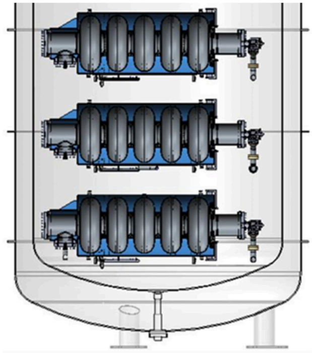
Figure 1: Schematic of STFC test system. Showing 3 cavities inside the cryostat.
