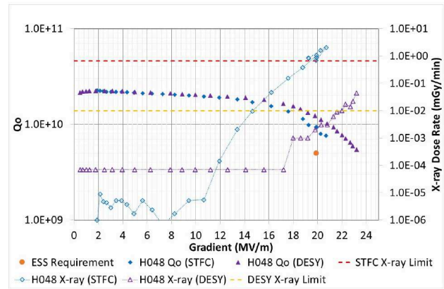
Figure 7: Radiation comparison of H048 at STFC and DESY.
