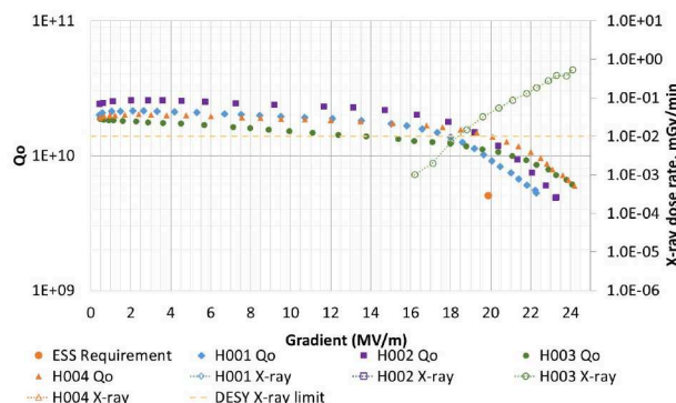
Figure 3: X Ray results H001 - H004 dressed cavity testing at DESY
