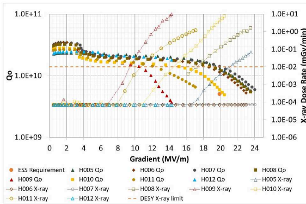
Figure 5: Production testing of cavities at DESY with a 12-hour HPR.
