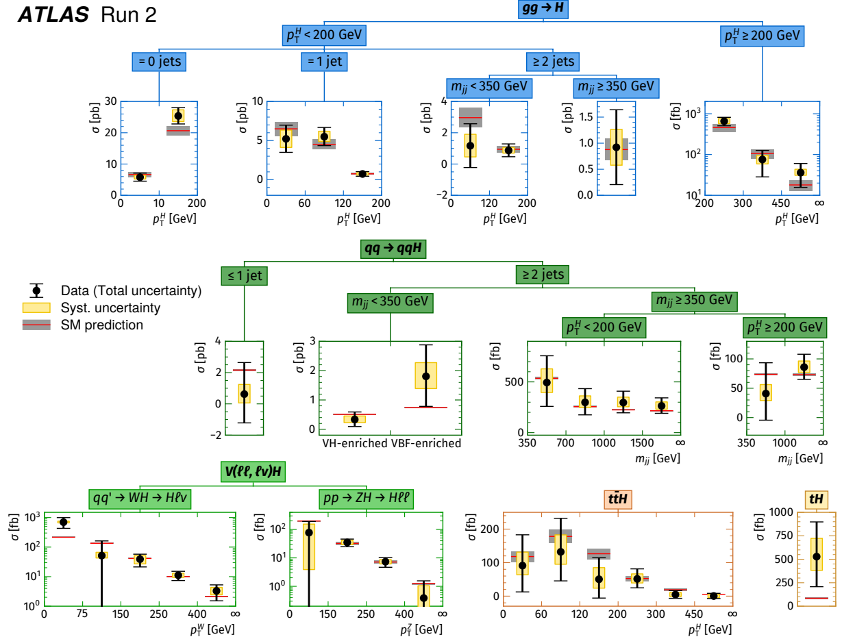
Figure 7: Observed and predicted Higgs boson production cross sections in different kinematic regions. The vertical bar on each point denotes the 68% confidence interval. The p -value for compatibility of the combined measurement and the SM prediction is 94%. Kinematic regions are defined separately for each production process, based on the jet multiplicity, the transverse momentum of the Higgs ( p_T^H ) and vector bosons ( p_T^W and p_T^Z ) and the two-jet invariant mass ( m_{jj} ). The ‘VH-enriched’ and ‘VBF-enriched’ regions with the respective requirements of m_{jj} \in [60, 120) GeV and m_{jj} \notin [60, 120) GeV are enhanced in signal events from VH and VBF productions, respectively.
