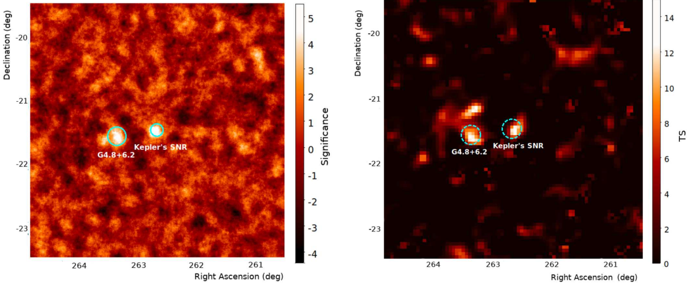
Fig. 1. H.E.S.S. and Fermi -LAT maps. Left panel: H.E.S.S. \gamma -ray significance map of Kepler's SNR using an oversampling radius of 0.1^\circ . Right panel: Fermi -LAT TS map in the range of 4.75–300 GeV. The position of Kepler's SNR is in the center of these maps. Solid circles in the left panel correspond to the source regions of Kepler's SNR and SNR G4.8+6.2 (to the east of Kepler's SNR), while dashed circles in the right panel merely indicate the locations of these SNRs. Neither of these sources are present in the 4FGL catalog.
