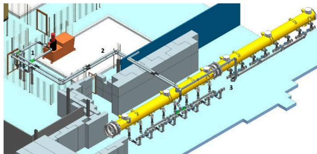
Figure 2: Overview of klystron- (1), connecting- (2) and cryomodule waveguide distribution (3) for ACC4 and ACC5.
