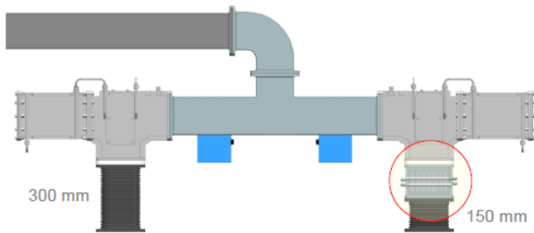
Figure 7: Position of the inserted attenuator for cavity 8 of ACC7.
