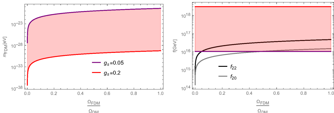
Figure 8. Predictions for the thraxion mass and decay constant as functions of the FDM abundance. All plots are drawn fixing M = 10 : increasing M makes the thraxions lighter. We then choose a conservative approach which allows us to have a wider phenomenology, given that the flux distribution in the landscape is an open field of investigation. For LVS, the volume scales as \mathcal{V} \sim e^{1/g_s} , hence allowing us to deal with only one free parameter (as we consider W_0 \sim \mathcal{O}(1) ).
