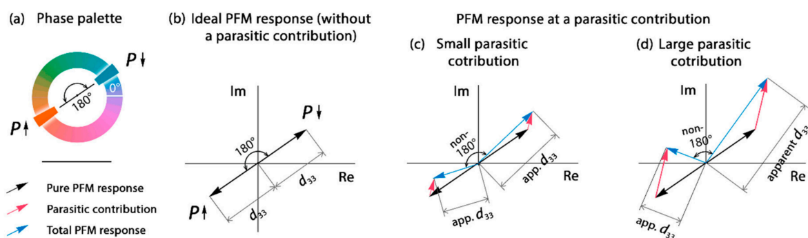
Figure 6. Complex PFM response for two polarization states and variations in the measured PFM phase and PFM amplitude at different conditions. (a) Phase palette used in Figure 3; (b) Ideal PFM response in the absence of parasitic contribution; PFM response at (c) small and (d) large parasitic contribution. Notation “ d_{33} ” means real d_{33} that was measured in PFM given the absence of a parasitic contribution. Notation “apparent d_{33} ” (“app. d_{33} ”) corresponds to the d_{33} measured when a parasitic contribution was present.
