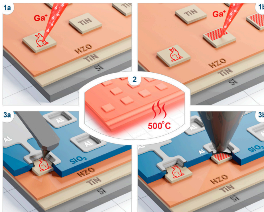
Figure 1. Design of the experiment. First step: The focused ion beam raster scans across the capacitor, implanting Ga ions either (1a) locally or (1b) homogeneously. Second (2) step: annealing takes place for crystallization of HZO (HZO) either into the ferroelectric phase or into the polymorphic state. Third step: Capacitors are addressed microscopically and macroscopically, either by a PFM study (3a) or electrophysical characterization at a probe station (3b).
