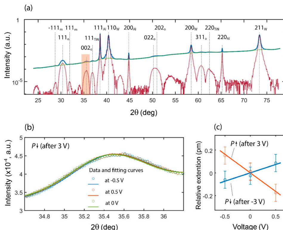
Figure 7. Measurement of the piezoelectric coefficient of the native HZO by in situ synchrotron X-ray microdiffractometry (micro-XRD). (a) Full spectrum (002 o peak is highlighted by orange; blue solid line is original spectrum, green solid line is a background, red dotted line is spectrum with subtracted background). (b) raw spectra and their fitting curves in the 2\theta range 34\text{--}36^\circ at different applied voltages; (c) relative extension of d -spacing for two monodomain polarization states.
