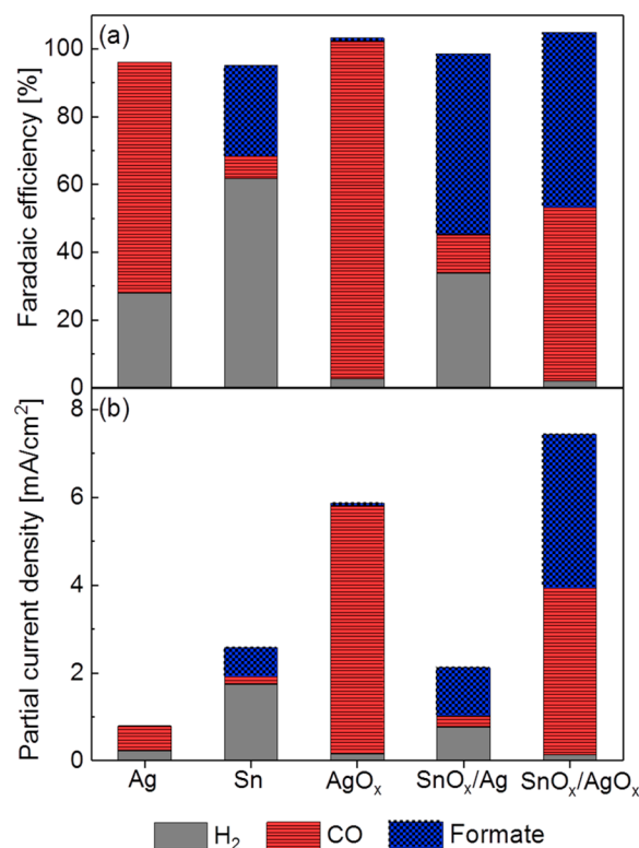
Figure 4. (a) Faradaic efficiencies and (b) partial current densities of \text{AgO}_x , \text{SnO}_x/\text{AgO}_x , \text{SnO}_x/\text{Ag} , metallic Ag, and Sn catalysts acquired after 1 h of \text{CO}_2\text{RR} at -0.8 V vs RHE in 0.1 M \text{KHCO}_3 . Each column represents Formate (dotted blue), \text{CO} (straight red line), and \text{H}_2 (gray).
