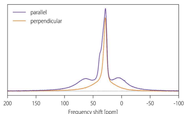
Fig. 8 The ^7\text{Li} NMR spectrum of the \text{LiC}_{5.8} sample recorded with the fiber axis oriented parallel (as for all other figures) and perpendicular to the magnetic field at 343 K. The intensity was normalized for better visualization of satellites.
