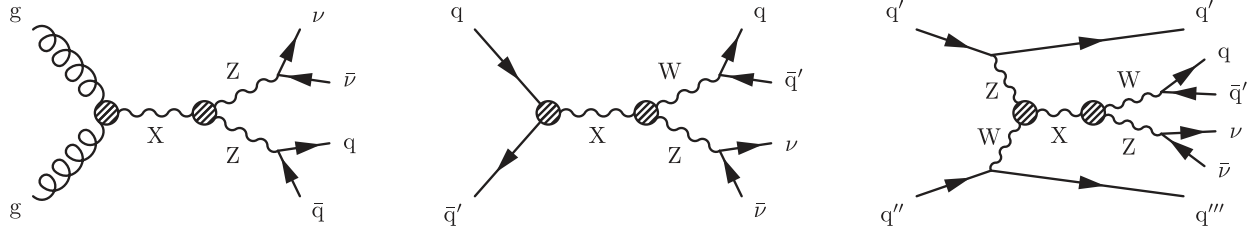
FIG. 1. Representative Feynman diagrams for various production modes of a heavy resonance X . These modes are: a ggF-produced spin-0 or spin-2 resonance decaying to ZZ \rightarrow q\bar{q}\nu\bar{\nu} (left), a DY-produced spin-1 resonance decaying to WZ \rightarrow q\bar{q}'\nu\bar{\nu} (center), and a VBF-produced spin-1 resonance decaying to WZ \rightarrow q\bar{q}'\nu\bar{\nu} (right).
