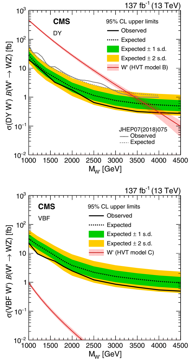
FIG. 9. Expected and observed 95% CL upper limits on the W' production cross section times the W' \rightarrow WZ branching fraction versus the W' mass are shown as dashed and solid black lines, respectively. Green and yellow bands, respectively, represent the 68% and 95% confidence intervals of the expected limit. The red curves show the theoretical W' boson production cross sections times their branching fractions to WZ . The hashed red areas represent the theoretical cross section uncertainty due to limited knowledge of PDFs and scale choices. Limits and theory cross sections for DY-produced W' bosons are shown in the left figure, while the right figure shows the same for VBF-produced W' bosons. The gray curves in the left plot show the previous CMS results with 36 \text{ fb}^{-1} of data.
