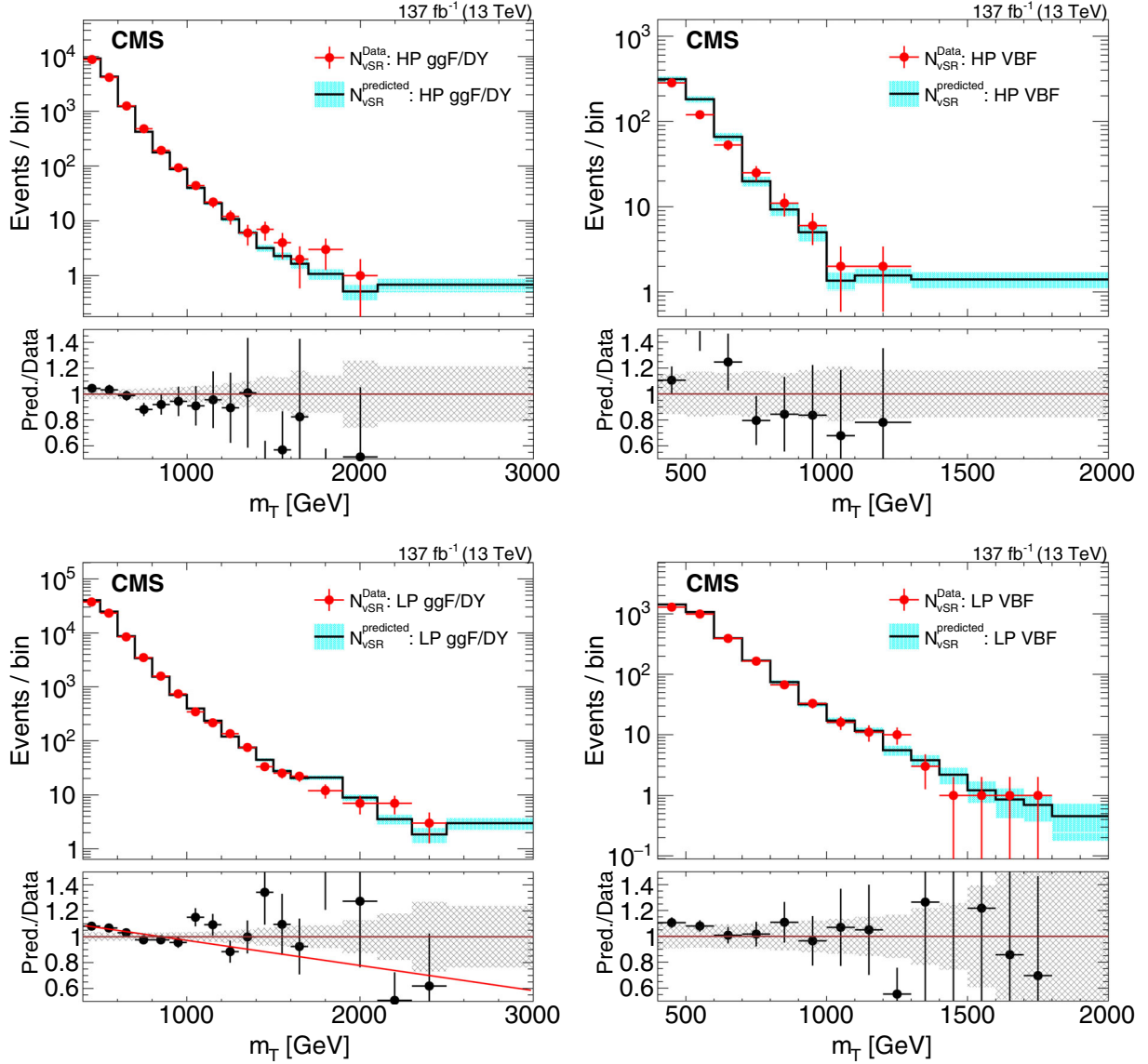
FIG. 5. Comparison of background estimations and observations in the high-purity ggF/DY (upper left), high-purity VBF (upper right), low-purity ggF/DY (lower left), and low-purity VBF (lower right) validation signal regions. The lower panel shows the ratio of the estimated and the observed event yields. The hashed band in the ratio represents the total uncertainty in the corresponding SR. The red line (lower left) is a fit to the ratio of prediction to the data in the LP ggF/DY vSR.
