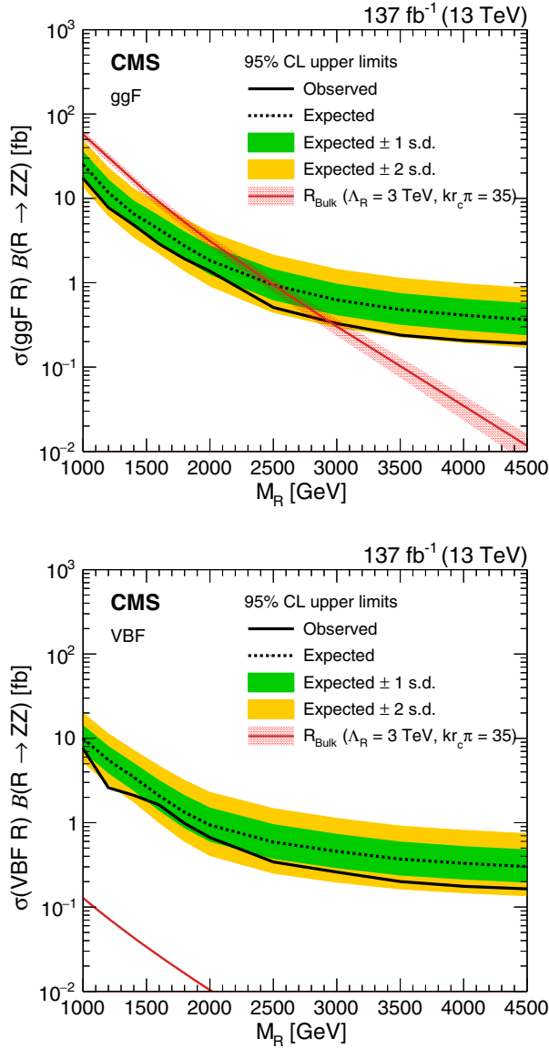
FIG. 8. Expected and observed 95% CL upper limits on the radion ( R ) production cross section times the R \rightarrow ZZ branching fraction versus the radion mass are shown as dashed and solid black lines, respectively. Green and yellow bands, respectively, represent the 68% and 95% confidence intervals of the expected limit. The red curves show the theoretical radion production cross sections times their branching fractions to ZZ . The hashed red areas represent the theoretical cross section uncertainty due to limited knowledge of PDFs and scale choices. Limits and theory cross sections for ggF-produced radions are shown in the left figure, while the right figure shows the same for VBF-produced radions.
