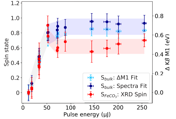
FIG. 3. The dependence of S_{\text{bulk}} as obtained by fitting of the \Delta M1 shift (light blue), and by fitting of the raw XES spectra to the reference spectra (dark blue) to the pulse energy of the incident XFEL beam. The \text{FeCO}_3 diffraction peak intensity ratio (red) estimates the spin state of \text{FeCO}_3 . The splitting of the blue and red shaded area above roughly 50 \mu\text{J} is due to the decomposition of \text{FeCO}_3 and shows the effect of Fe bearing decomposition products on the spin state S_{\text{bulk}} .
