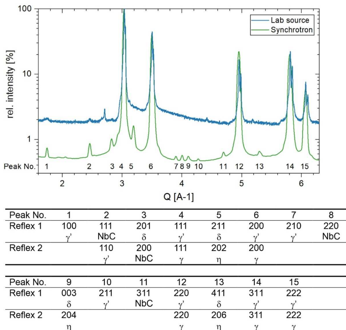
Figure 2. Room temperature diffraction pattern measured with lab-source and synchrotron X-rays. On the bottom, a list of selected indexed diffraction peaks for the different phases is shown.
