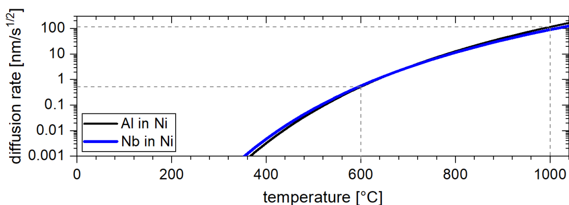
Figure 12. Calculated diffusion rate for aluminum and niobium in nickel. The diffusion rate was calculated by an Arrhenius equation and literature data for Al [40] and Nb [41] in Ni.
