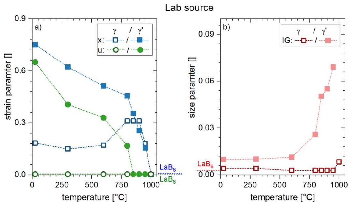
Figure 9. Evolution of (a) the strain parameter (u, x) and (b) the size parameter (IG) with rising testing temperature for the lab-source XRD experiments. The dashed lines next to the diagrams indicate the instrumental strain and size parameter, which were measured by LaB6. A higher strain or size parameter may be related to an increasing lattice strain or decreasing crystallite size, respectively.
