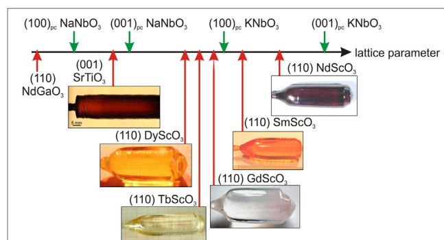
FIGURE 1 | Schematic presentation of the pseudocubic (pc) lattice parameters of \text{NaNbO}_3 and \text{KNbO}_3 (end members of the solid-solution K_x\text{Na}_{1-x}\text{NbO}_3 ) as well as the average in-plane lattice parameters of different perovskite-like substrate surfaces. The rare-earth scandates \text{ReScO}_3 ( \text{Re} = \text{Dy}, \text{Tb}, \text{Gd}, \text{Sm}, \text{Nd} ) are all grown at the Leibniz Institute for Crystal Growth (Uecker et al., 2006, 2008, 2013; Coh et al., 2010; Gugushev et al., 2015). A part of the figure is reproduced from Gugushev et al. (2015) with permission from the Royal Society of Chemistry.
