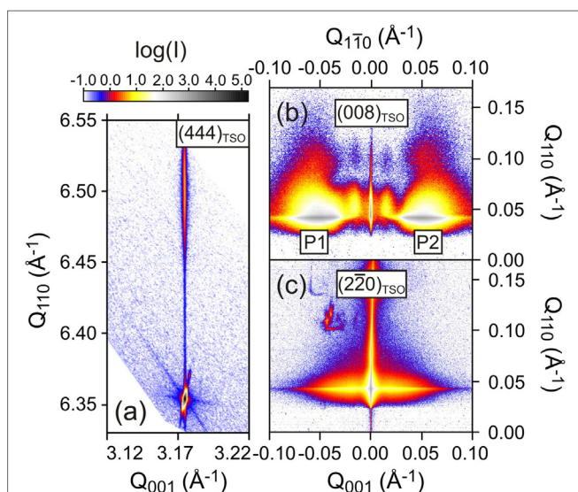
FIGURE 5 | (A) X-ray reciprocal space maps around the (444) TSO substrate Bragg reflection. Grazing incidence in-plane X-ray diffraction map in the vicinity of (008) TSO (B) and (220) TSO (C) substrate Bragg reflections.
