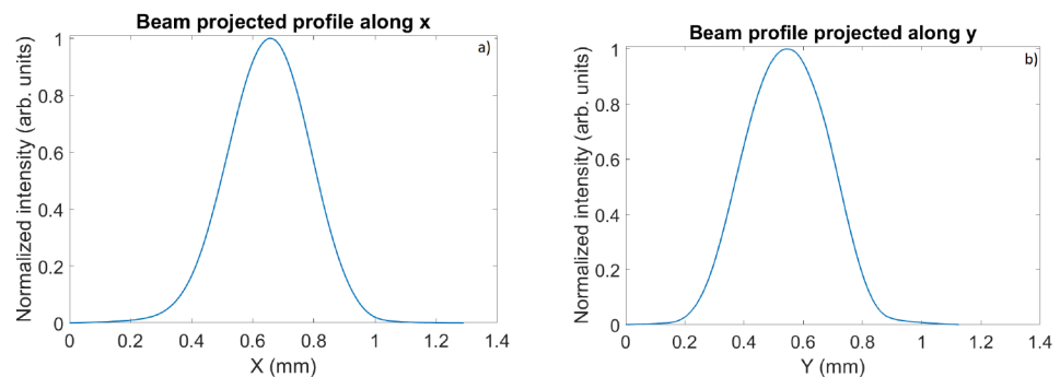
Figure 10. Analysis of the beam profile along x (a) and y directions (b).
