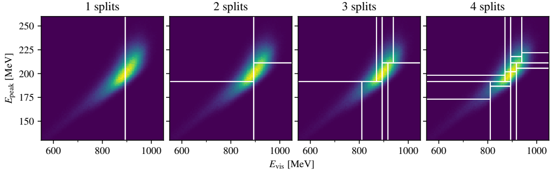
Figure 5. Quantiles developing by splitting the validation set of into subsets of equal size regarding their energy sum & peak energy.
