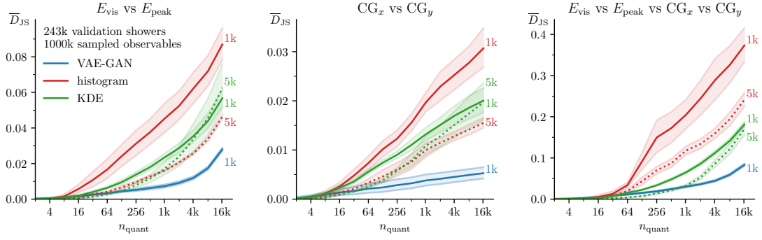
Figure 10. Dependence of \bar{D}_{JS} on the number of quantiles n_{\text{quant}} for 1000k observable values sampled from different density estimators for multi-dimensional combinations of the observables given in eq. (2.2), in analogy to the 1D results in figure 9.
