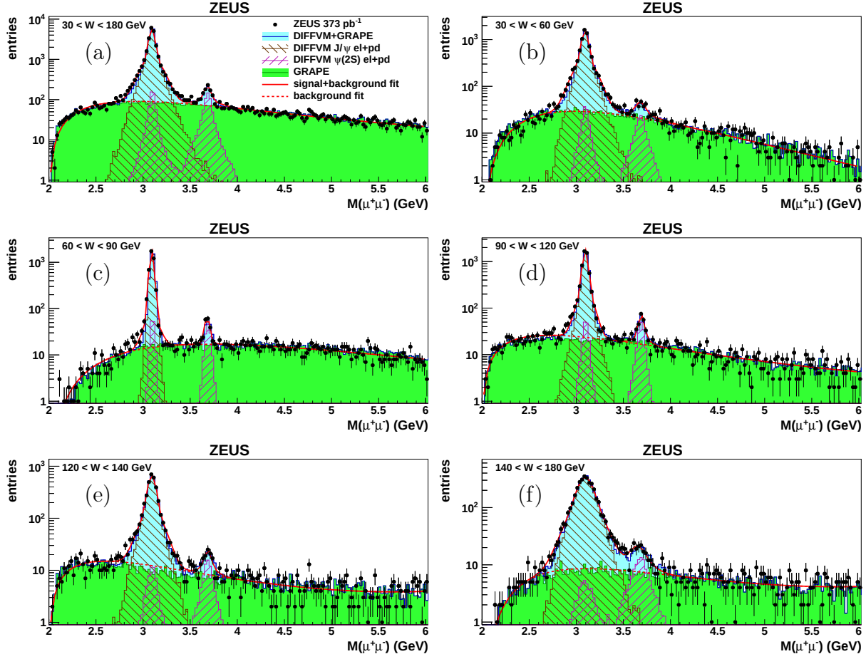
Figure 2: Measured invariant mass distribution, M(\mu^+\mu^-) , of dimuon pairs (solid circles) in selected photoproduction events with error bars denoting statistical uncertainties. The data are shown in (a) the full W range, 30 < W < 180 GeV, and (b) – (f) finer W intervals within the full range. Monte Carlo distributions for simulated events are shown for DIFFVM elastic and proton-dissociative processes of J/\psi(1S) (brown hatched histogram) and \psi(2S) (purple hatched histogram) and for a continuous background of muon pairs (GRAPE, green solid histogram) from the Bethe–Heitler process. The solid blue histogram represents the sum of all processes. The relative contribution of different processes was obtained from a fit to the data in the range 2 < M(\mu^+\mu^-) < 6 GeV. The result of a double-Gaussian fit to the resonant peaks and parameterisation of the background, described in the text, is also shown (solid and dashed lines).
