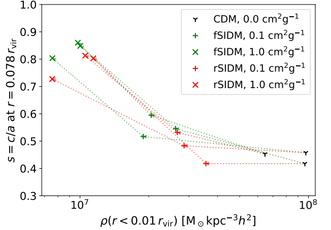
Figure 15. The shape within an ellipsoid with the volume of a sphere with a radius of r = 0.078 r_{\text{vir}} is shown as a function of the central density within a sphere of r = 0.01 r_{\text{vir}} for individual systems. The colours indicate the type of self-interactions and the symbols give their strength. We show the three most massive haloes ( \sim 1.2\text{--}1.7 \times 10^{14} M_{\odot} h^{-1} ) of the highest resolved full box simulation at a redshift of z = 0 . How they evolve when increasing the cross-section is indicated by the arrows.
