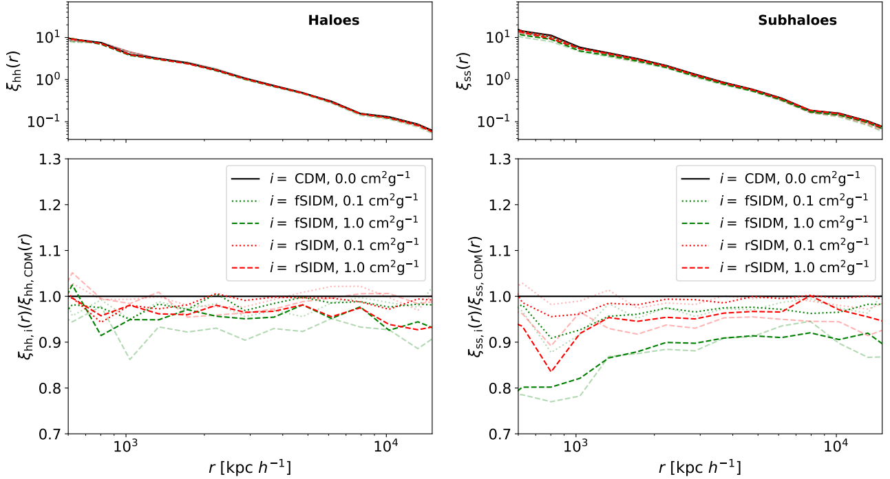
Figure 4. The two-point correlation function is shown for the higher resolution boxes (uhr, darker lines) and the lower resolution boxes (hr, fainter lines). For the left panel, we used the halo positions and computed the halo-halo correlation, \xi_{hh}(r) . Likewise, we used the subhalo positions and computed the subhalo-subhalo correlation, \xi_{ss}(r) , as displayed in the right panel. Note that we only considered haloes and subhaloes that have at least a mass of \sim 9.6 \times 10^{10} M_{\odot} h^{-1} . Results for various DM models, as indicated in the legend, are shown for a redshift of z = 0 .
