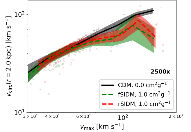
Figure 11. The circular velocity at 2 kpc vs. the maximum circular velocity measured from the circular velocity profile as shown in Fig. 10 is displayed. Each dot corresponds to one of the 300 most massive subhaloes of the highest resolved zoom-in simulation. The lines correspond to the mean and the shaded regions indicate the standard deviation.
