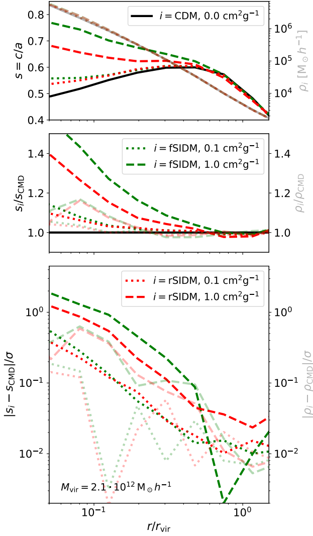
Figure D1. In the upper row, we display the median density (transparent) and shape profiles for the lowest halo mass bin (as in the bottom panels of Fig. 8, 12 and 13) of our uhr simulations at z = 0 . The median mass of the haloes is 2.1 \times 10^{12} M_{\odot} h^{-1} . In the middle row, we show the ratio between the SIDM models and CDM. We further compute the difference of the SIDM models and CDM and divide it by the scatter among the individual systems. The result is displayed in the bottom row. The x -axis is in terms of the radius that a spherical shell with the same volume has. Here we use the mean of the two shell boundaries.
