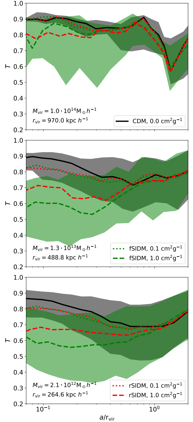
Figure 13. The same as in Fig. 12 but we show the triaxiality T instead of s = c/a . The triaxiality is computed according to Eq. (5).
