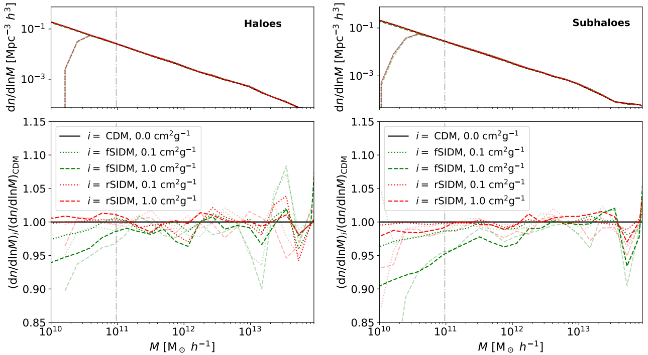
Figure 5. The halo mass (left panel) and the subhalo mass (right panel) function are shown for various simulations. We plot the number density of haloes/subhaloes per logarithmic mass bin as a function of the total halo/subhalo mass as identified by SUBFIND. The colours indicate the type of the self-interaction and the line style gives the strength of self-interaction as indicated in the legend. We display results of the higher resolution boxes (uhr, darker lines) and the lower resolution boxes (hr, fainter lines). The dash-dotted grey line indicates the mass limit of \sim 9.6 \times 10^{10} M_{\odot} h^{-1} that we applied previously for the two-point correlation function. The plots are for a redshift of z = 0 .
