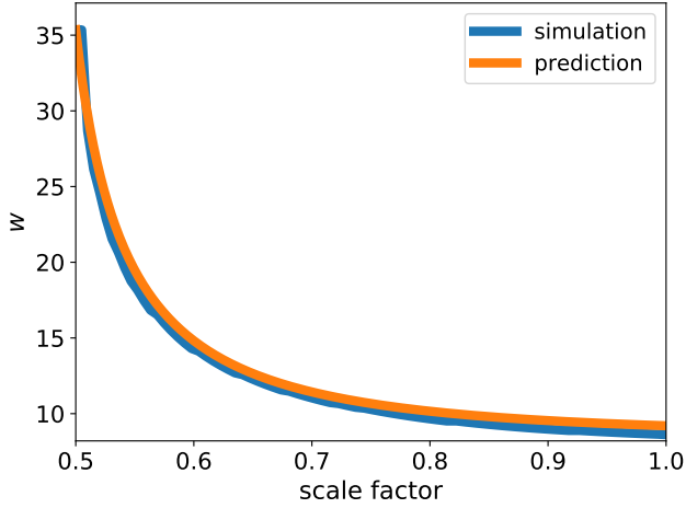
Figure A1. The cosmic deceleration problem in terms of the canonical momentum is shown. It is simulated from a = 0.5 to a = 1.0 with 122500 particles in a cubic box with a comoving side length of 1400 \text{ kpc } h^{-1} . The total mass is 22.8465 \times 10^{10} M_{\odot} h^{-1} , corresponding to a comoving density of 83.26 M_{\odot} \text{ kpc}^{-3} h^2 . The initial snapshot velocity of the test particle is 100 \text{ kpc Gyr}^{-1} , which corresponds to an initial canonical momentum of 35.35534 \text{ kpc Gyr}^{-1} . The particles are evolved with a cross-section of \sigma_{\tilde{T}}/m_{\chi} = 5 \times 10^5 \text{ cm}^2 \text{ g}^{-1} and the SIDM kernel sizes are computed using N_{\text{ngb}} = 64 .
