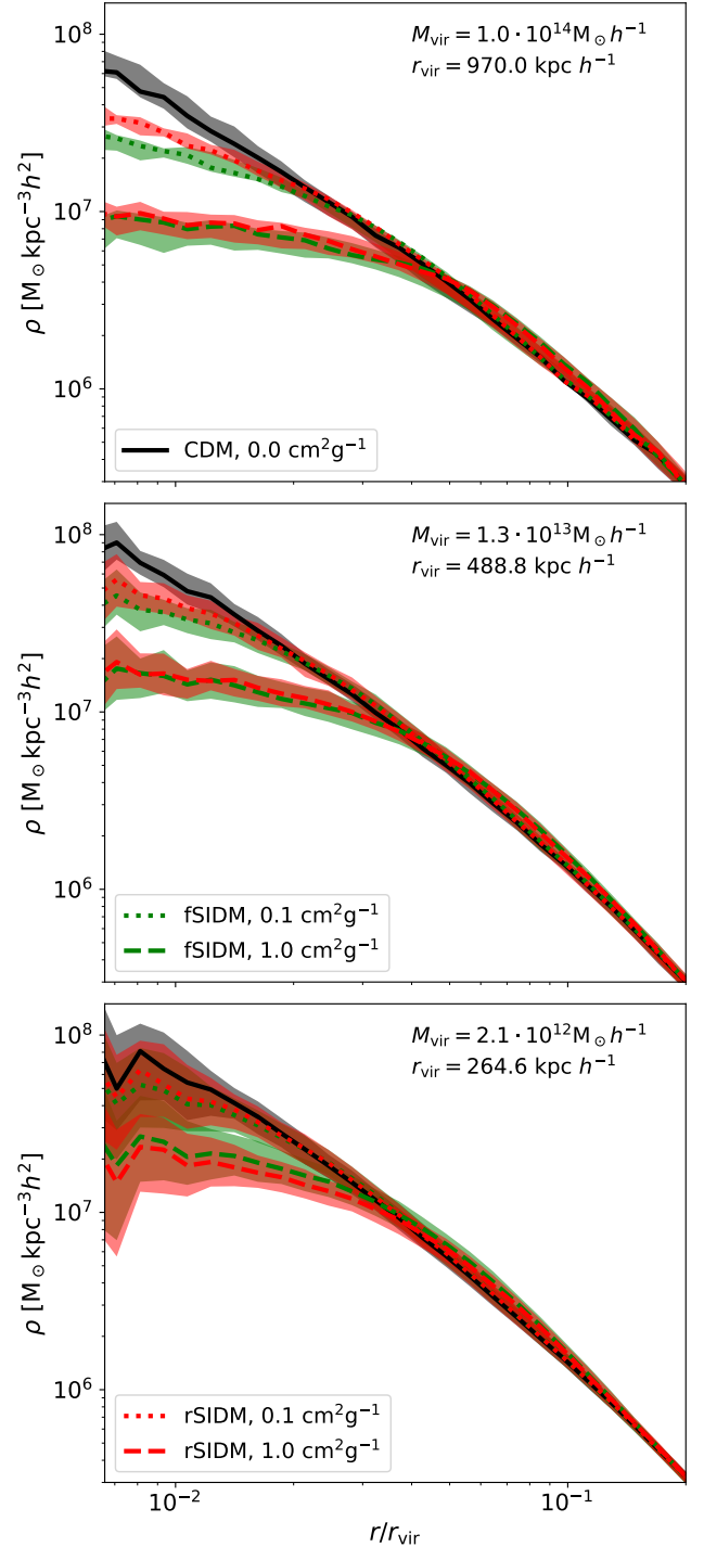
Figure 8. Median density profiles are shown for various halo mass bins and cross-sections. The density is plotted as a function of the radius in units of the virial radius. The shaded regions indicate the scatter among the haloes, the range between the 25th and 75th percentiles is displayed. The virial mass and the virial radius given in the panels indicate the median of the corresponding mass bin. All plots show the profiles for a redshift of z = 0 and are produced from the full cosmological box with the highest resolution. Note, we have used all particles, not only those that belong to the halo as identified by SUBFIND.
