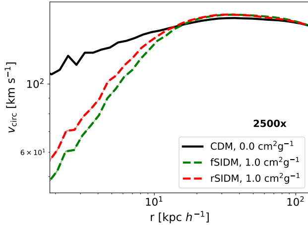
Figure 10. The circular velocity as a function of radius is shown for the most massive subhalo of our highest resolved zoom-in simulation at a redshift of z = 0 .
