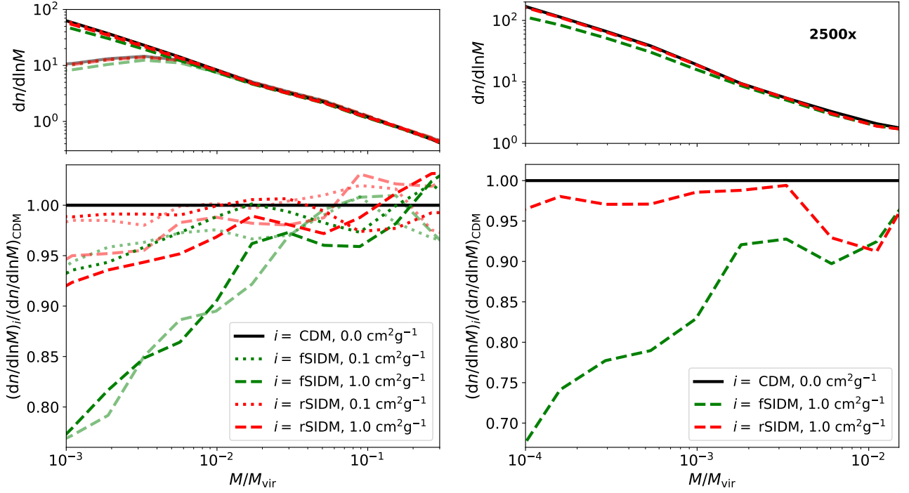
Figure 6. The number of satellites per logarithmic mass as a function of their total mass relative to the virial mass of their host. The left panel gives the result of the 100 most massive groups in our full cosmological box with the highest resolution and the lower resolution run (transparent). The right panel gives the same but for the three most massive objects in the best resolved zoom-in simulation. All subhaloes, except for the primary one, that are within a radius of 5 r_{\text{vir}} were considered satellites. The results are for a redshift of z = 0 . Note, the least resolved satellites of the uhr and x2500 simulations used here contain about 100 particles.
