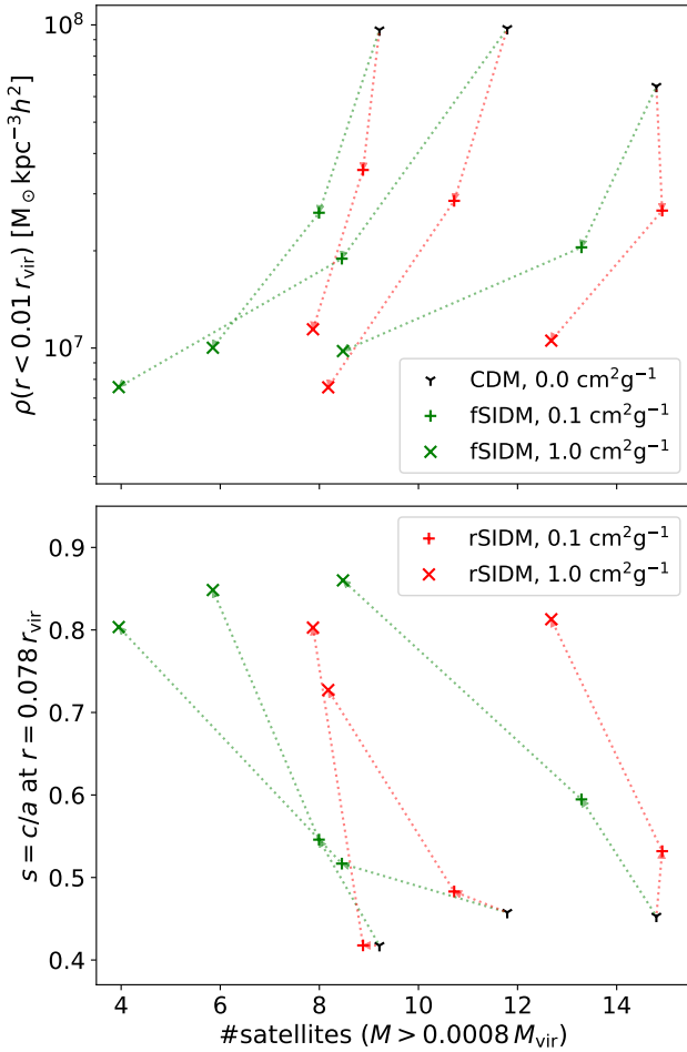
Figure 16. We show the 3 most massive haloes of our full box simulation at z = 0 , the same as in Fig. 15. The upper panel gives the central density within a radius of 0.01 r_{\text{vir}} as a function of the number of satellites and the lower panel gives the shape of an ellipsoid that has the same volume as a sphere with an radius of 0.078 r_{\text{vir}} as a function of the number of satellites. For the satellite count, only satellites within r_{\text{vir}} and with a mass larger than 0.0008 M_{\text{vir}} were considered. This implies that every satellite is at least resolved by \geq 2200 particles. The arrows connect the same systems across the simulations with various cross-sections.
