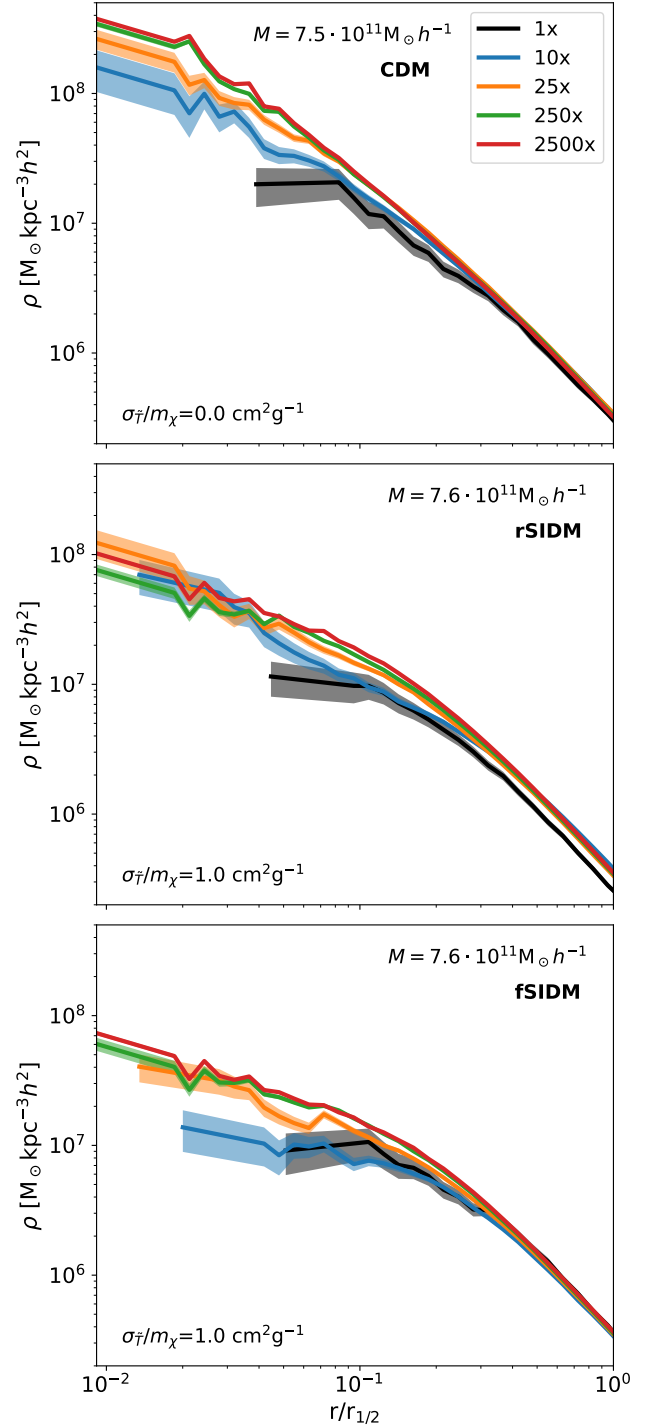
Figure B1. The density profile of the most massive subhalo in our zoom-in simulation is shown. In the top panel, we display the results for CDM, in the middle panel for rSIDM and the bottom panel for fSIDM. The colours indicate runs with different resolutions, further details can be found in Tab. 2. In the highest resolution run the halo is resolved by \sim 2.3 \times 10^6 particles.
