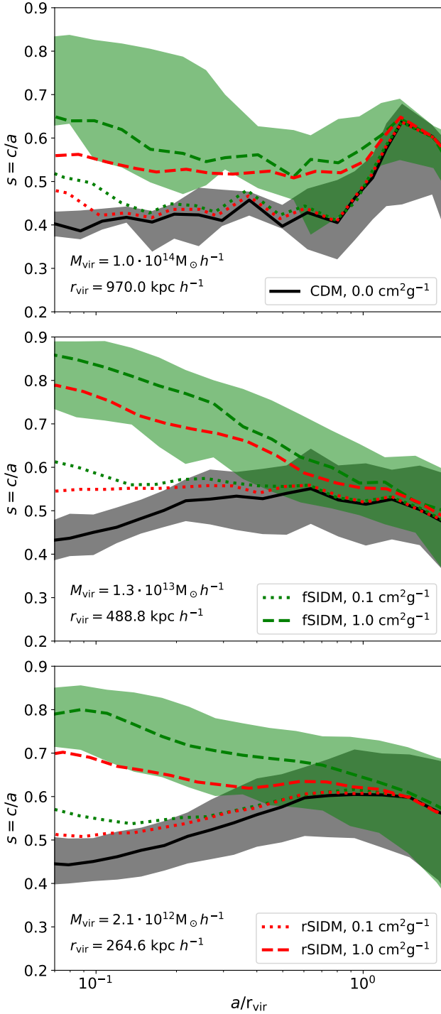
Figure 12. The median halo shapes for different mass bins are shown as a function of the median semi-major axis in units of the virial radius. We compute the median shape as well as the median semi-major axis from ellipsoids having the same volume. The shaded regions indicated the scatter among the haloes, the range between the 25th and 75th percentiles is displayed. For the sake of clarity, we show this only for the CDM simulation and the fSIDM run with the larger cross-section. The virial mass given in the panels indicates the median virial mass of the haloes of the corresponding mass bin. The same applies to the shown virial radius. Note, we are using the same mass bins as in Fig. 8. The shapes are computed from the highest resolved full cosmological box and for a redshift of z = 0 .
