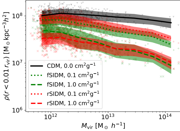
Figure 9. We display the central density of haloes as a function of their virial mass. The results of various simulations at a redshift of z = 0 are shown. The central density is measured as the mean density within a sphere of 0.01 r_{\text{vir}} . Systems evolved with the smaller cross-section are marked by “+” and for the larger cross-section we use “x”, the CDM case is indicated by “y”. In addition to the individual systems, we computed the mean of the distribution as a function of virial mass, indicated by the lines. The shaded region gives the standard deviation.
