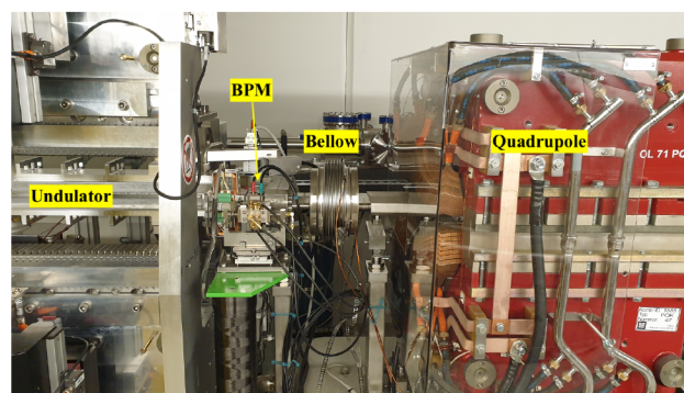
Figure 2: Bellow installed in the tunnel downstream of an undulator (left) followed by a BPM and upstream of a girder (right) carrying a red quadrupole.
