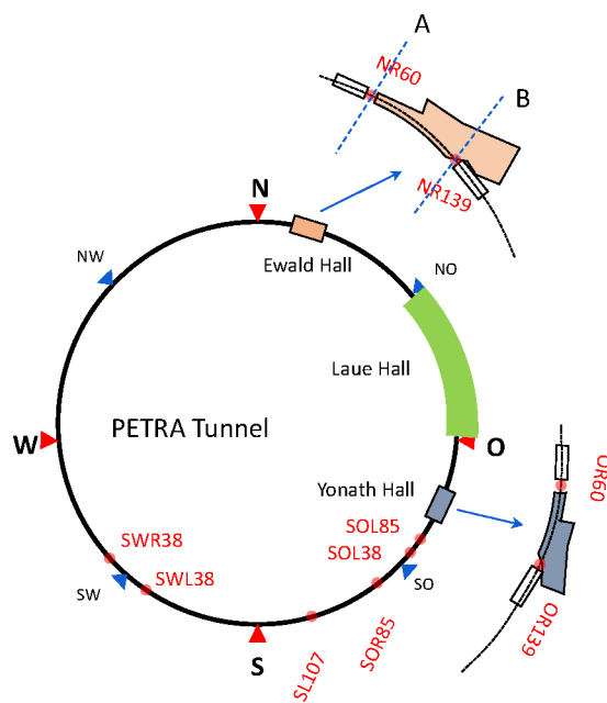
Figure 1: Overview of the PETRA III tunnel layout with its three experimental halls, indicating the locations of the mechanical measurement devices shown in Fig. 2 (right).
