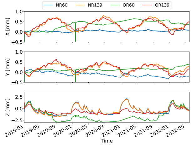
Figure 4: Measured movement at the four stations on the extremities of the two extension experimental halls (Paul Ewald Hall and Ada Yonath Hall), exact locations are indicated in Fig. 1.
