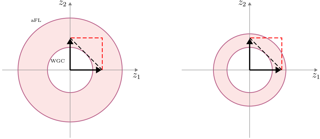
Figure 1: Convex shell: allowed axionic states should lay inside the red area, between the inner (WGC) and the outer (aFL) circle. On the left, the charge vectors satisfy both conjectures, while on the right we have a violation of the aFL bound. Indeed, charge vectors need to be big enough for all extremal dyonic black holes (inner circle) to decay, so that the black dotted line lies outside the circle. If we also impose aFL and in a situation where the outer shell is very thin, having very big charge vectors could violate the aFL bound. In the right-hand side plot, the basis charge vectors barely satisfy aFL while the (1, 1) charge vector violates it.
