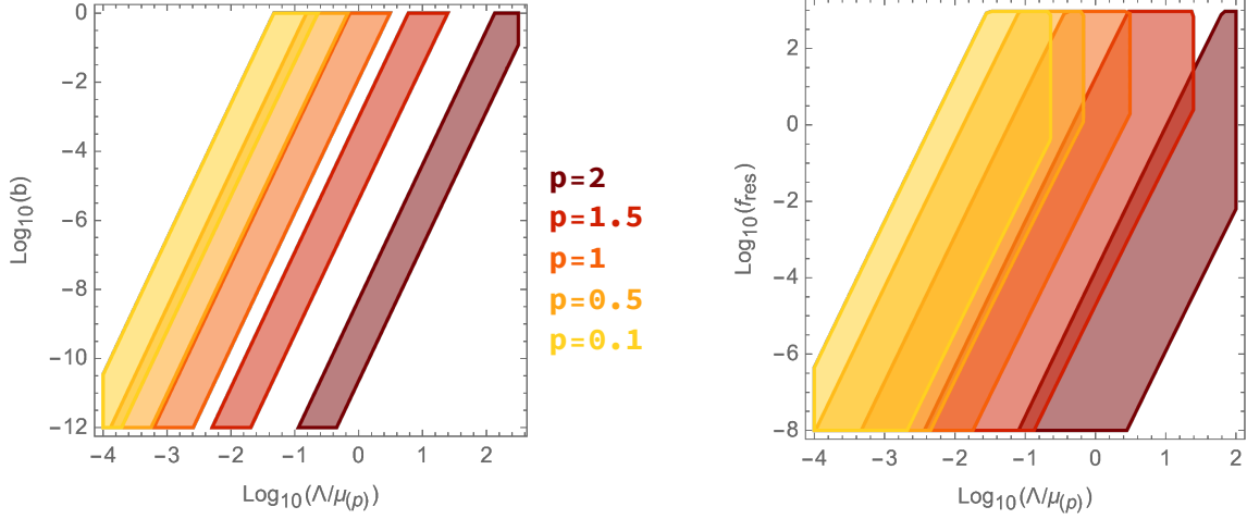
Figure 2: Theoretically allowed values of b^* (left) and f_{NL}^{\text{res}} (right) coming from imposing monotonicity of the inflationary potential, i.e., b^* < 1 , FL and WG conjectures, and requiring that \omega^* < 10^2 to match experimental constraints [41]. These results refer to the monomial monodromy potential in Eq. (3.1), fixing the number of e-folding in absence of wiggles to be N = 50 and imposing COBE normalization.
