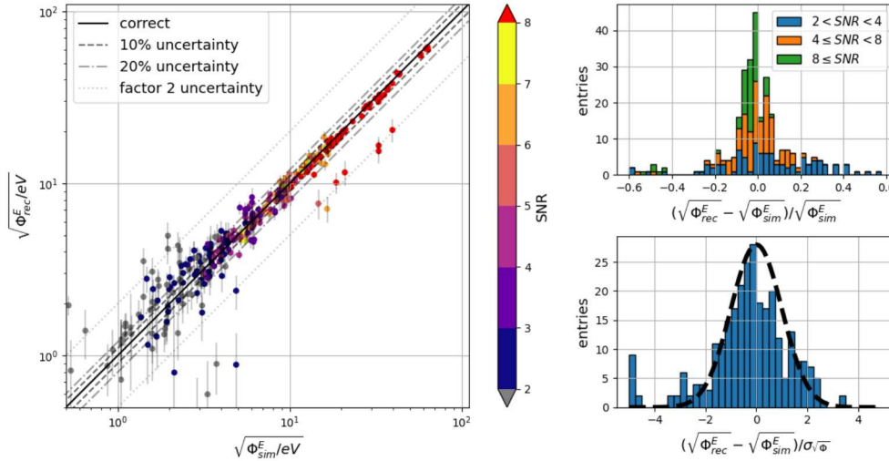
Figure 12. Reconstruction of energy fluence of the radio signals from inclined air showers detected with an ARIANNA-like radio detector at the site of the Pierre Auger Observatory. Left: Scatter plot of the reconstructed square root of the energy fluence \sqrt{\Phi^E} vs. the actual energy fluence of the radio signal. The errorbars show the uncertainty estimated by the IFT reconstruction algorithm. Top right: Stacked histogram of the errors of the reconstructed \sqrt{\Phi^E} for different signal-to-noise ratios. Bottom right: Errors of the reconstructed \sqrt{\Phi^E} as a multiple of the estimated uncertainty. For comparison, a Gaussian function with \sigma = 1 is drawn as well. The left- and rightmost bins in each histogram are overflow bins.
