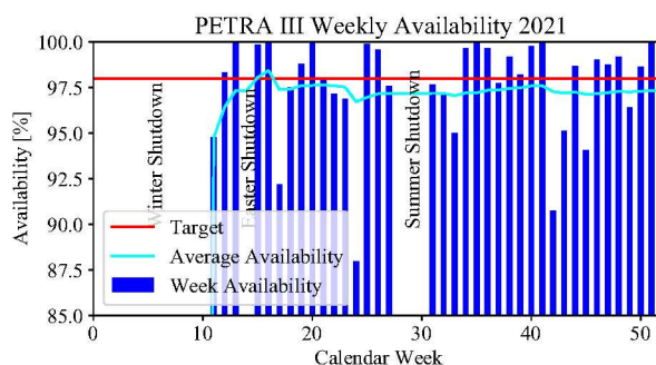
Figure 3: PETRA III availability per calendar week in 2021.
