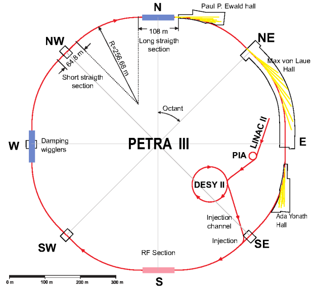
Figure 1: Layout of PETRA III.
