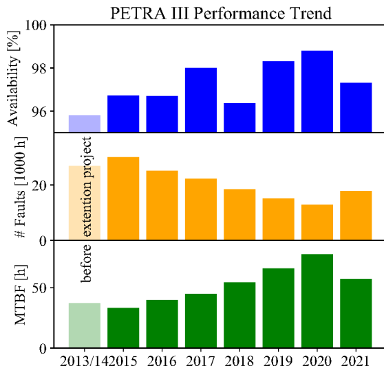
Figure 5: PETRA III performance trend. Top: availability, middle: number of faults per 1000 h, bottom: MTBF. All quantities are given during user run time only.
