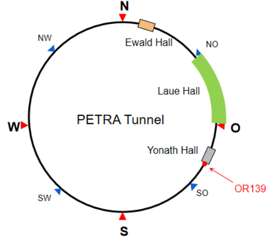
Figure 1: Overview of the PETRA III tunnel layout. Location OR139 (139 m right of East hall) is highlighted (red) as the location of the tunnel motion measurement presented in Fig. 2.
