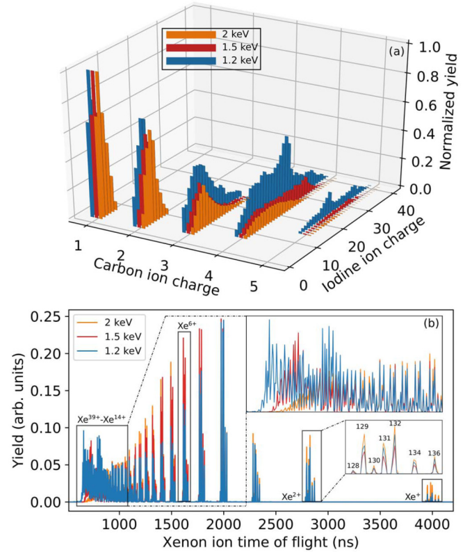
FIG. 1. (a) Charge state distributions of [\text{I}^{m+}, \text{C}^{n+}] ion pairs produced by ionization of \text{CH}_3\text{I} molecules with x rays at 2 keV, 1.5 keV, and 1.2 keV. The normalization is performed by scaling the maximum yield value of the charge state distribution to one. (b) Time-of-flight spectra of xenon ions produced by ionization of xenon atoms with x rays under the same conditions as in the molecular case. The inset at the top right magnifies the region of high charge states above \text{Xe}^{14+} . The seven \text{Xe}^{2+} peaks and their associated isotope masses (in amu) are shown by the inset at the bottom right. Also labeled are \text{Xe}^{+} and \text{Xe}^{6+} peaks.
