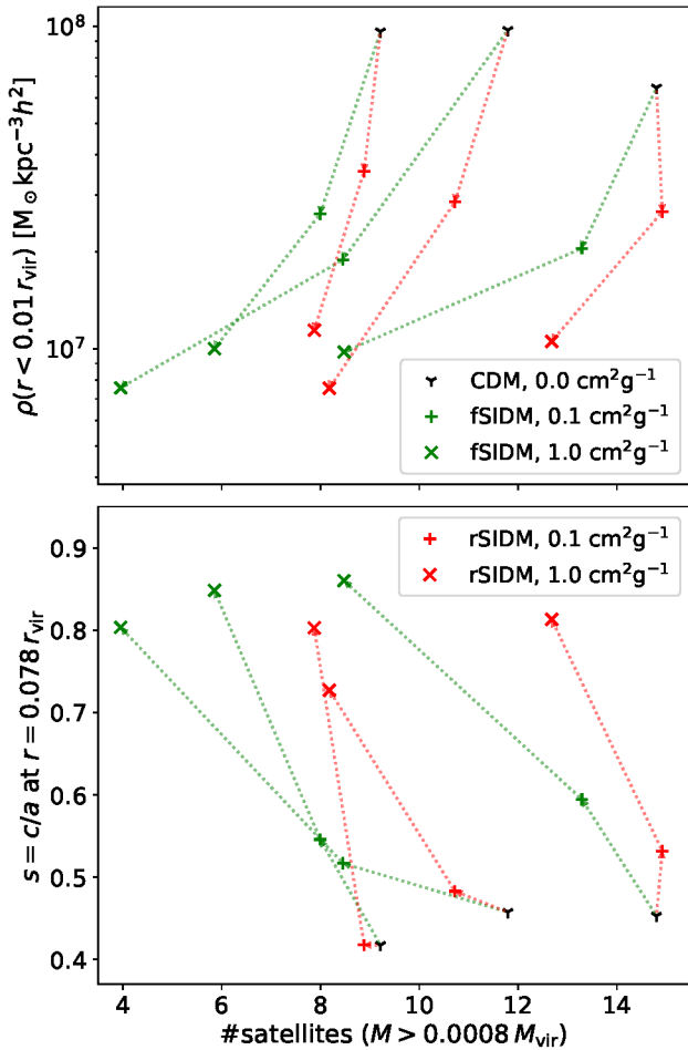
Figure 16. We show the 3 most massive haloes of our full box simulation at z = 0 , the same as in Fig. 15. The upper panel gives the central density within a radius of 0.01 r_{\text{vir}} as a function of the number of satellites and the lower panel gives the shape of an ellipsoid that has the same volume as a sphere with an radius of 0.078 r_{\text{vir}} as a function of the number of satellites. For the satellite count, only satellites within r_{\text{vir}} and with a mass larger than 0.0008 M_{\text{vir}} were considered. This implies that every satellite is at least resolved by \geq 2200 particles. The arrows connect the same systems across the simulations with various cross-sections.
