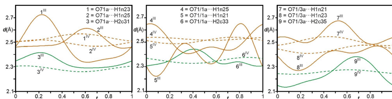
Figure 8. t-Plots of the interatomic distances (Å) between the oxygen atoms of nitrate group A and hydrogen atoms of the Co(sep) cage involved in N–H...O bonds (orange) and C–H...O bonds (green) in phase III (full curves) compared to those in phase IV [9c] (dashed curves). A similar plot for nitrate group B is given in Supporting Information, Figure S7.
