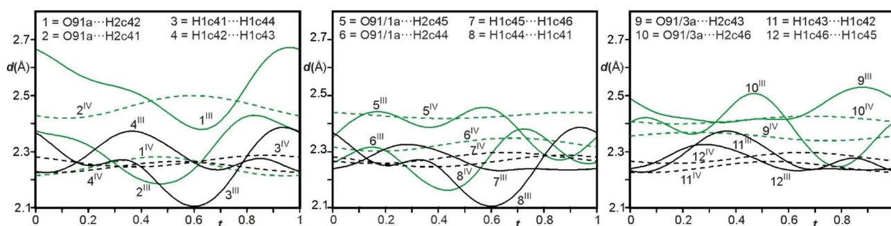
Figure 9. t-Plots of the interatomic distances (Å) between the oxygen atoms of nitrate group C and Co(sep) cage involved in C–H...O bonds (green); and between hydrogen atoms of adjacent Co(sep) cages (black) in phase III (full curves) compared to those in phase IV [9c] (dashed curves).
