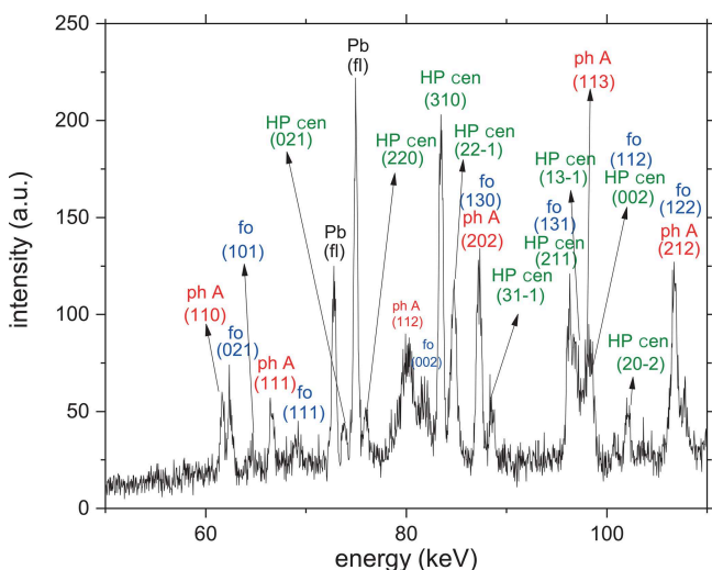
Figure 4. X-ray diffraction obtained in situ at 9.8 GPa and 750 °C from run 502 (Table 1).
