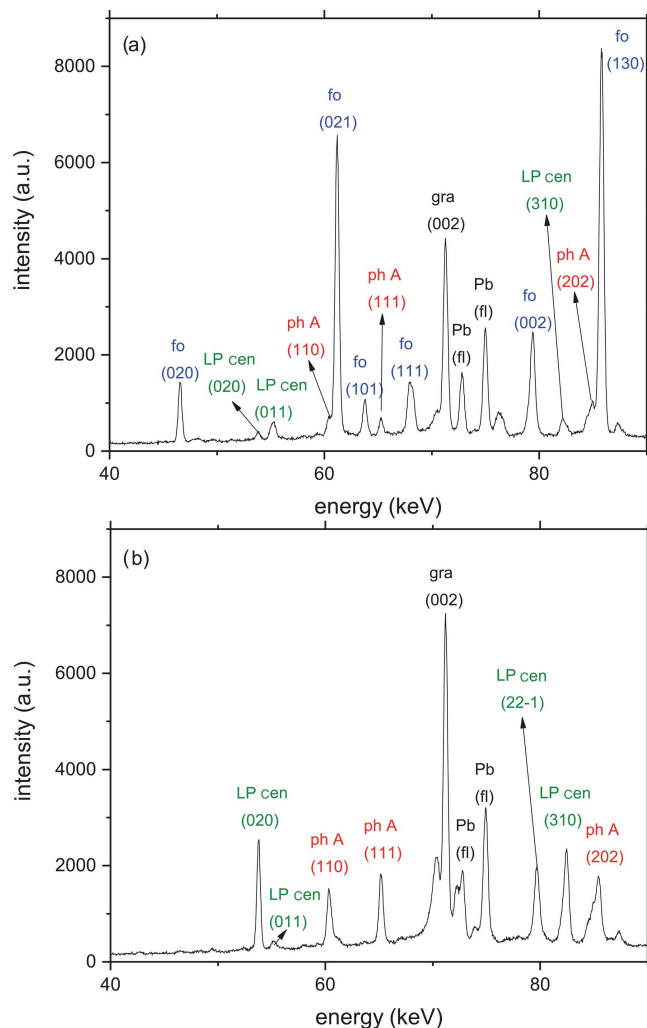
Figure 2. (a) Representative diffraction patterns of the starting material for all reversal experiments taken at room T and ambient P in situ in the multi-anvil press. Beside the X-ray reflections of the starting materials forsterite (fo), phase A (ph A), and low P clinoenstatite (LP cen), additional reflections relate to the (002) graphite (gr) peak at 71.3 keV from the heater and Pb fluorescence (fl) at 74.96 and 72.80 keV from the detector shielding. (b) Representative diffraction pattern of the starting material for all kinetic experiments at room P and T , containing ph A and LP cen, together with the (002) graphite peak and the two Pb fluorescence lines.
