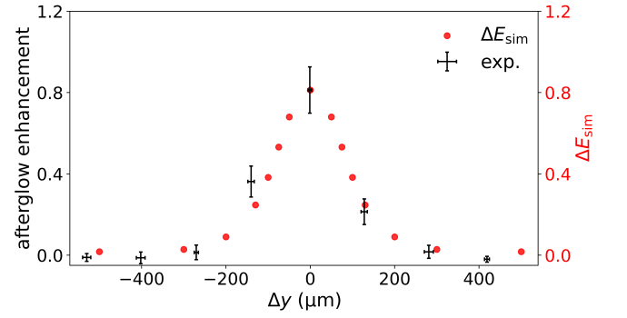
FIG. 4: Spatial alignment scan with 8-10 shots per setting with experimentally observed plasma afterglow enhancement (black) and normalized energy transfer obtained from simulation (red).
