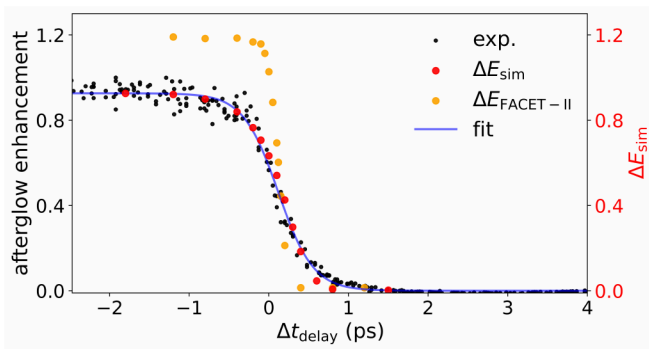
FIG. 5: Experimental time-of-arrival scan over 256 consecutive shots within -2.5 \text{ ps} < \Delta t_{\text{delay}} < 4.0 \text{ ps} . Black: experimental normalized afterglow enhancement. Blue: sigmoid fit for experimental data. Red: normalized energy transferred into the plasma from PIC simulations. Orange: a FACET-II-class beam yields a substantially steeper transition.
