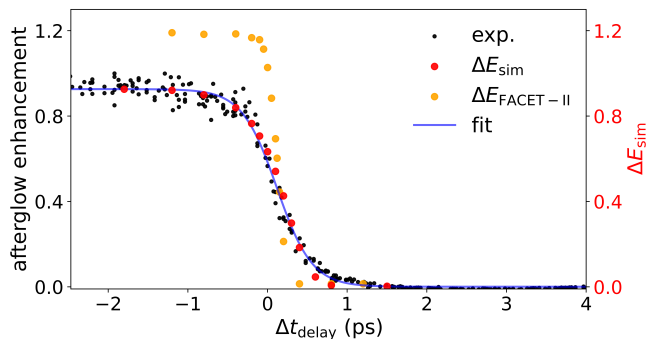
FIG. 5: Experimental time-of-arrival scan over 256 consecutive shots within -2.5 \text{ ps} < \Delta t_{\text{delay}} < 4.0 \text{ ps} . Black: experimental normalized afterglow enhancement. Blue: sigmoid fit for experimental data. Red: normalized energy transferred into the plasma from PIC simulations. Orange: a FACET-II-class beam yields a substantially steeper transition.
