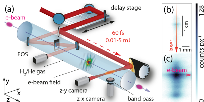
FIG. 1: Experimental setup and afterglow shots: (a), The electron beam propagates through gas and couples with an overlapping laser-generated seed plasma. (b), Example of laser-only plasma afterglow at 587 nm. (c), Example of electron-beam enhanced plasma afterglow.
