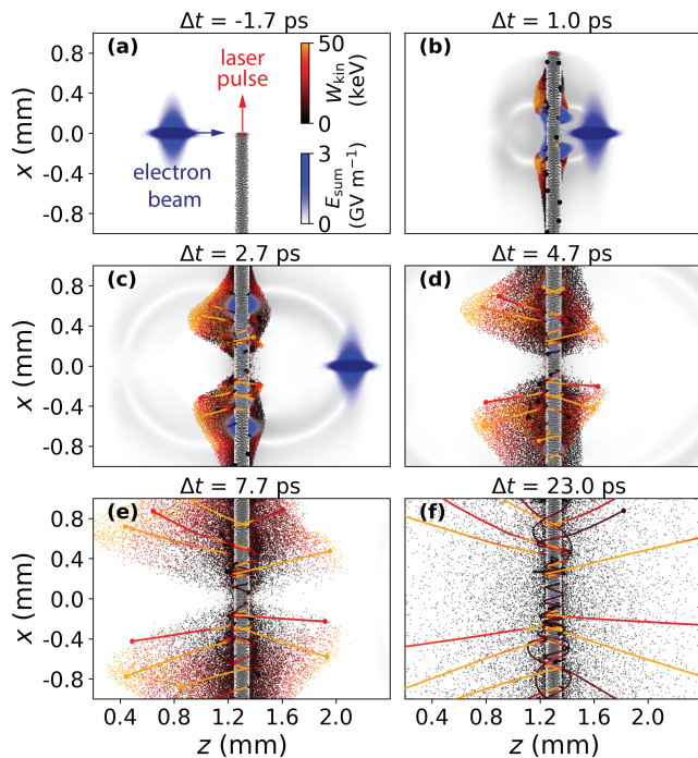
FIG. 2: PIC-simulation snapshots. (a), The electron beam approaches the emerging laser-generated H 2 /He plasma filament (black dots), reaching the filament center at \Delta t = 0 . (b, c), The electron beam crosses the filament and heats plasma electrons via its unipolar transverse field (blue). Plasma surface waves (blue, central slice of simulation) propagate along the filament and transport density perturbations. (b-f), Localized plasma electron oscillations visualized by typical electron trajectories (solid lines), color-coded by momentary energy.
