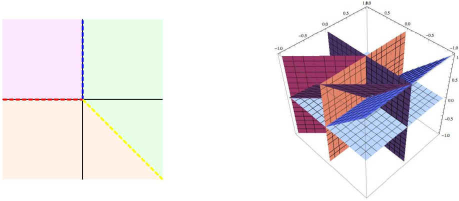
Figure 9. Left: The \langle 1346 \rangle tropical hypersurface, given by the half-planes (in the transverse x_3 direction) (x_1 = 0, x_2 > 0) , (x_1 = -x_2, x_2 < 0) , (x_2 = 0, x_1 < 0) where \min(0, x_1, x_1 + x_2) is attained twice simultaneously. From ref. [189]. Right: The Tr_+(4, 6) fan.
