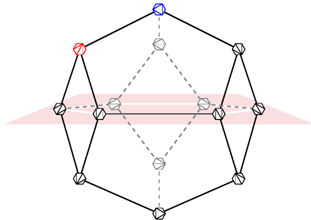
Figure 3. The cluster polytope of the Gr(4,6) \simeq A_3 cluster algebra, with clusters representing the different triangulations of a hexagon, as discussed in the text and in figure (2), where also the vertex labels may be found. The initial and mutated cluster in the left- and right-hand side of figure 1 are color-coded in red and blue, respectively. The parity invariant plane is also drawn in pink. Adapted from refs. [108, 23].
