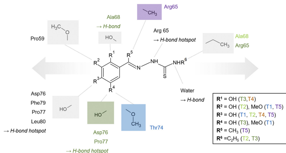
FIGURE 7 | Generic and schematic binding model of the thiosemicarbazones core structure based on the investigated derivatives. Selected PLpro amino acids participating in hydrophobic interaction and hydrogen bonds are displayed and additionally color-coded if they are only relevant for one of the compounds. Conserved and individual hydrogen bond positions are labeled. Moieties, which are exclusively present in one compound, are color-coded, e.g., the methoxylation in the position of R^4 is exclusive for T1 and colored blue accordingly. The proposed options to extend the thiosemicarbazone compounds, either at the phenyl ring or at the terminal nitrogen of the thiourea moiety, are indicated schematically by arrows.
