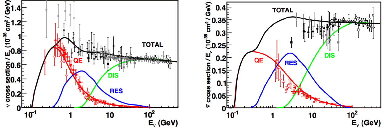
FIG. 4: Comparison of neutrino (left) and anti-neutrino (right) cross sections. Data is from [894] and the theory calculations are from [895]. The figure is reproduced from [896].
