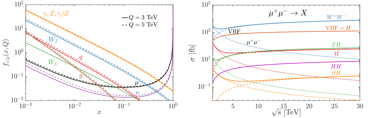
FIG. 2: The distributions for the EW PDFs (left) and the corresponding predictions for a few representative SM processes at a high-energy muon collider (right). Adapted from Ref. [825].
