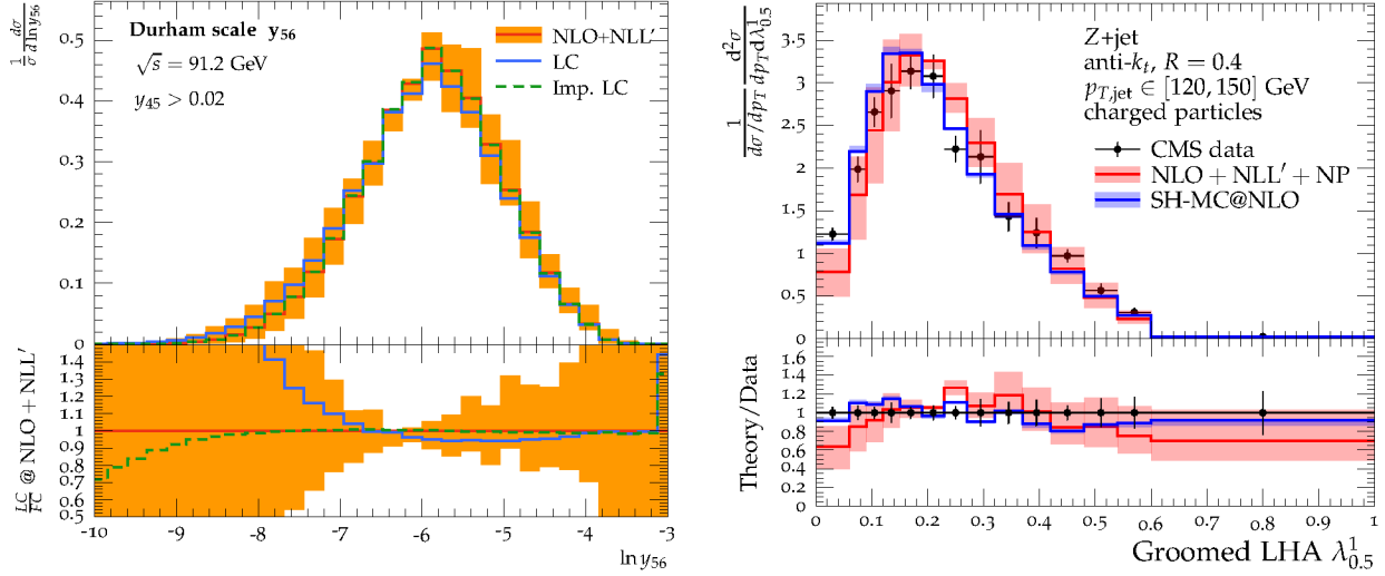
FIG. 3: Left: Durham jet resolution scale y_{56} describing the 5 \rightarrow 6 jet transition, at NLO+NLL' compared to various simplified color treatments. Right: Les Houches angularity \lambda_{0.5}^1 of the leading jet in Z+jet production, including the effect of soft drop grooming. Data from CMS compared to the NLO+NLL'+NP prediction and a full SHERPA simulation.
