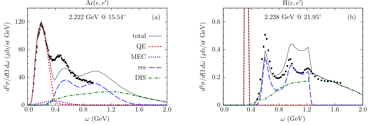
FIG. 7: Comparison of the predictions of GENIE 2.12 for the double differential cross sections for electron scattering on (a) argon and (b) hydrogen with the data [1113–1115], as reported in Ref. [888].
