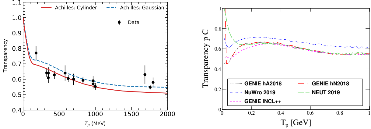
FIG. 6: Carbon transparency as a function of the kicked proton kinetic energy. Left: Shows results for ACHILLES for the cylinder and Gaussian interaction models compared to data from [982–987], figure is reproduced from [970]. Right: Shows results from GENIE hA2018, GENIE hN2018, NEUT 2019, NuWro 2019, GENIE INCL++, figure is reproduced from [971].
