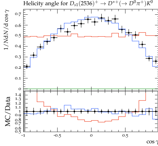
FIG. 9: Efficiency-corrected normalized signals as functions of \cos \gamma in comparison to experimental data from BELLE [1345]. Green Histograms show default predictions from HERWIG, while red and blue histograms are respectively predictions with only the implementation of HQEFT and with HQEFT effects in the presence of improved hadronization and decay models.
