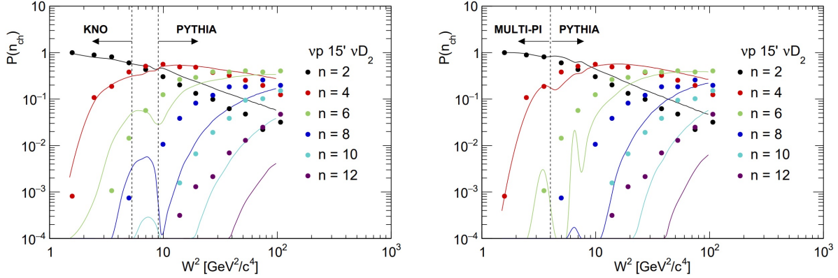
FIG. 5: Data-MC comparisons for normalized topological cross-sections for muon neutrino - proton scatterings. The left is from GENIE v3 (tune G18_02a_02.11a) [953] and the right is from the NEUT v5.4.0.1 [954]. Data are from the Fermilab 15' bubble chamber [955]. MC simulations show large non-physical discontinuities of topological cross-sections and these simulations suggest event-by-event predictions of hadronic final states are extremely challenging using current methods.
