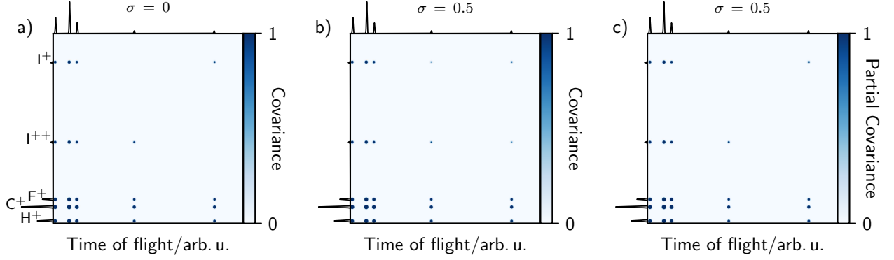
FIG. 4. Time-of-flight covariance maps produced from simulated Coulomb explosions of 3,5-difluoriodobenzene into atomic ions over 5000 laser shots, with v=20 and \sigma=0 (a) or 0.5 (b). The experimental variance introduces false correlations between I^+ and I^{2+} , which can be removed using a partial covariance correction (c). Each covariance map is normalized to its maximum value.
