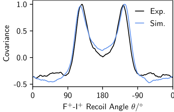
FIG. 3. Experimental (black) and simulated (blue) \text{F}^+ \text{-I}^+ angular distributions from the analogous \text{Cov}(\text{I}^+, \text{F}^+) images in Figure 2.
