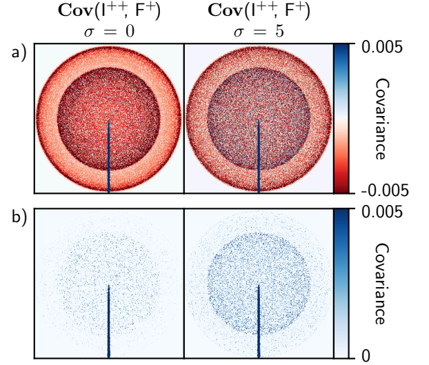
FIG. 5. (a) Recoil-frame covariance images produced from simulated Coulomb explosions of 3,5-difluoriodobenzene into two channels: F^+ and I^+ , or F^+ and I^{2+} . Each image was produced with v=20 and \sigma=0 or 5. The increase in \sigma produces false correlations between the two channels, which appear as two positive isotropic features at high and low kinetic energies. (b) The positive components of the covariance. Each image is normalized to its maximum value.
