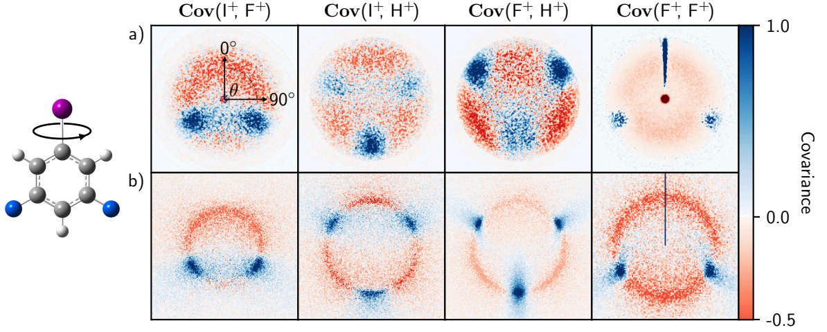
FIG. 2. Recoil-frame covariance images \text{Cov}(\mathbf{A}, \mathbf{B}) of fragment pairs produced from the experimental (a) and simulated (b) Coulomb explosions of 3,5-difluoriodobenzene molecules aligned along their carbon-iodine bond axes. Each displays the velocity distribution of a fragment ion B relative to a reference ion A recoiling at 0^\circ . The experimental images were created from the data used in reference 9. 9 The predicted images were simulated from 5,000 laser shots using the model described in the text with an event rate of 10 and perfect detection efficiency.
