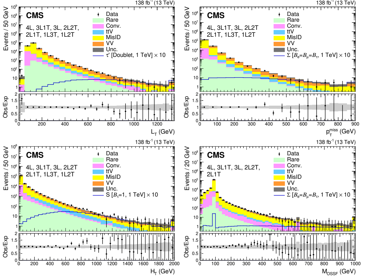
Figure 5: The distributions of L_T (upper left), p_T^{\text{miss}} (upper right), and H_T (lower left) in all seven multilepton channels, and M_{\text{OSSF}} (lower right) in channels with at least one light lepton pair (4L, 3L1T, 3L, 2L2T, and 2L1T). The rightmost bin contains the overflow events in each distribution. The lower panel shows the ratio of observed events to the total expected background prediction. The gray band on the ratio represents the sum of statistical and systematic uncertainties in the SM background prediction. As illustrative examples, a signal hypothesis for the production of the vector-like \tau lepton in the doublet scenario of m_{\tau'} = 1 TeV and a scalar leptoquark coupled to a top quark and a \tau lepton of m_S = 1 TeV are overlaid in the L_T and H_T distributions respectively. Similarly, a signal hypothesis for the production of the type-III seesaw heavy fermions in the flavor-democratic scenario of m_\Sigma = 1 TeV is overlaid for the p_T^{\text{miss}} and M_{\text{OSSF}} distributions.
