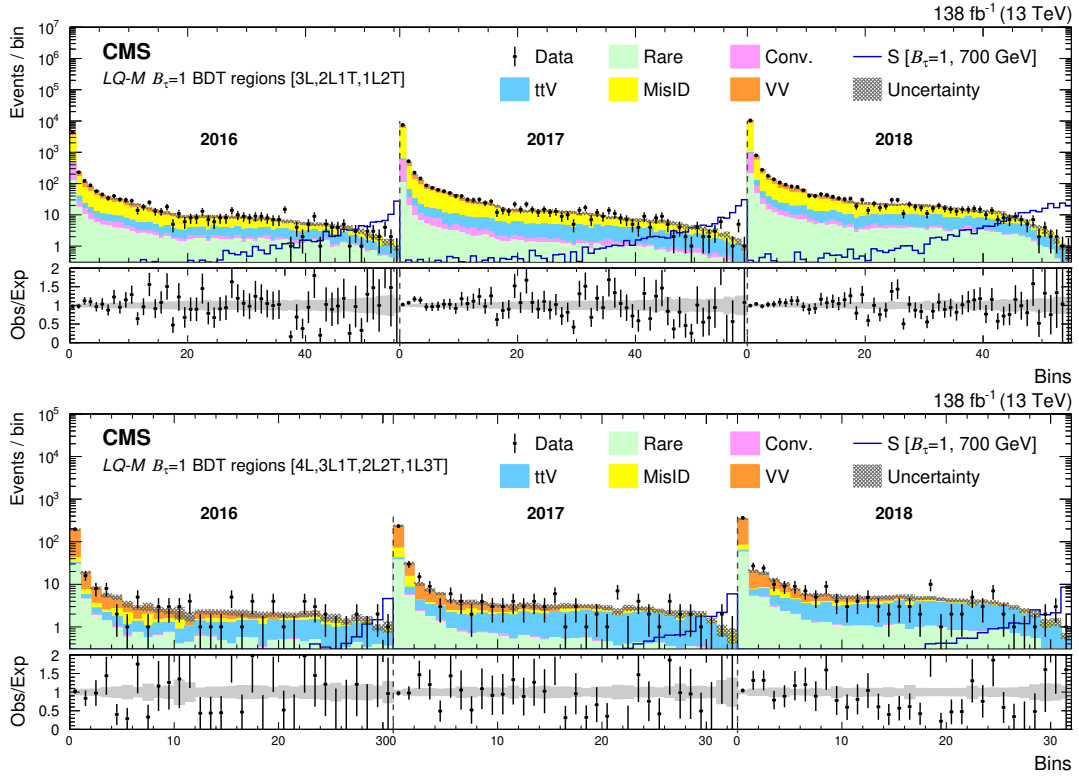
Figure 19: The LQ-M B_\tau = 1 BDT regions for the 3-lepton (upper) and 4-lepton (lower) channels for the 2016–2018 data sets. The lower panel shows the ratio of observed events to the total expected background prediction. The gray band on the ratio represents the sum of statistical and systematic uncertainties in the SM background prediction. The expected SM background distributions and the uncertainties are shown after fitting the data under the background-only hypothesis. For illustration, an example signal hypothesis for the production of the scalar leptoquark coupled to a top quark and a \tau lepton for m_S = 700 \text{ GeV} , before the fit, is also overlaid.
