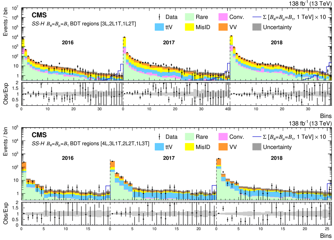
Figure 14: The SS-H \mathcal{B}_e = \mathcal{B}_\mu = \mathcal{B}_\tau BDT regions for the 3-lepton (upper) and 4-lepton (lower) channels for the 2016–2018 data sets. The lower panel shows the ratio of observed events to the total expected background prediction. The gray band on the ratio represents the sum of statistical and systematic uncertainties in the SM background prediction. The expected SM background distributions and the uncertainties are shown after fitting the data under the background-only hypothesis. For illustration, an example signal hypothesis for the production of the type-III seesaw heavy fermions in the flavor-democratic scenario for m_{\Sigma} = 1 TeV, before the fit, is also overlaid.
