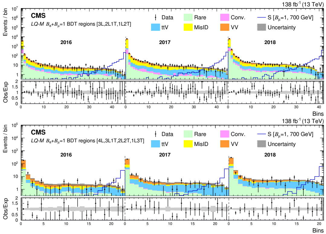
Figure 21: The LQ\text{-}M \mathcal{B}_e + \mathcal{B}_\mu = 1 BDT regions for the 3-lepton (upper) and 4-lepton (lower) channels for the 2016–2018 data sets. The lower panel shows the ratio of observed events to the total expected background prediction. The gray band on the ratio represents the sum of statistical and systematic uncertainties in the SM background prediction. The expected SM background distributions and the uncertainties are shown after fitting the data under the background-only hypothesis. For illustration, an example signal hypothesis for the production of the scalar leptoquark coupled to a top quark and a muon for m_S = 700 GeV, before the fit, is also overlaid.
