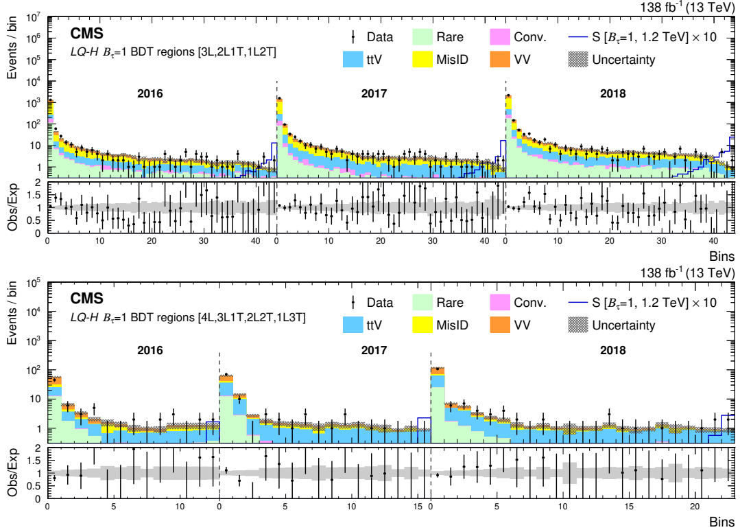
Figure 20: The LQ-H B_\tau = 1 BDT regions for the 3-lepton (upper) and 4-lepton (lower) channels for the 2016–2018 data sets. The lower panel shows the ratio of observed events to the total expected background prediction. The gray band on the ratio represents the sum of statistical and systematic uncertainties in the SM background prediction. The expected SM background distributions and the uncertainties are shown after fitting the data under the background-only hypothesis. For illustration, an example signal hypothesis for the production of the scalar leptoquark coupled to a top quark and a \tau lepton for m_S = 1.2 \text{ TeV} , before the fit, is also overlaid.
