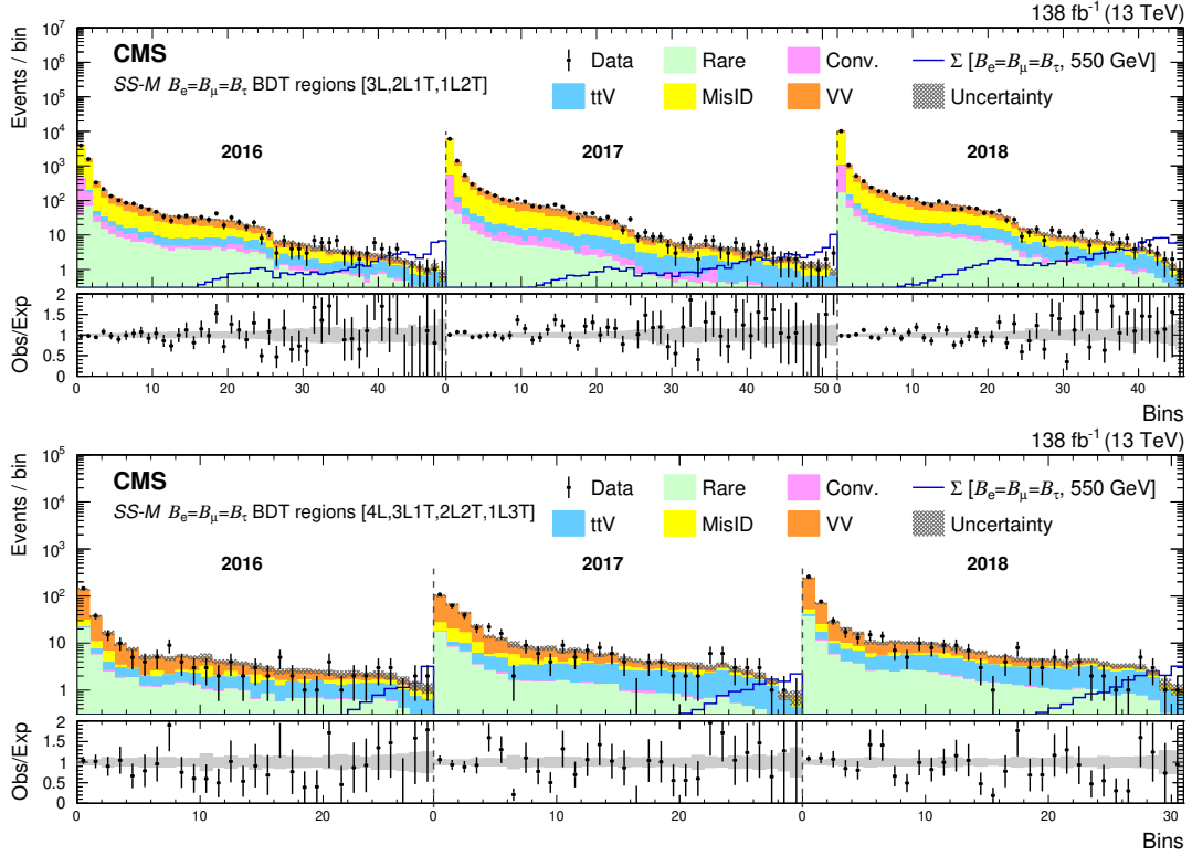
Figure 13: The SS\text{-}M B_e = B_\mu = B_\tau BDT regions for the 3-lepton (upper) and 4-lepton (lower) channels for the 2016–2018 data sets. The lower panel shows the ratio of observed events to the total expected background prediction. The gray band on the ratio represents the sum of statistical and systematic uncertainties in the SM background prediction. The expected SM background distributions and the uncertainties are shown after fitting the data under the background-only hypothesis. For illustration, an example signal hypothesis for the production of the type-III seesaw heavy fermions in the flavor-democratic scenario for m_\Sigma = 550 \text{ GeV} , before the fit, is also overlaid.
