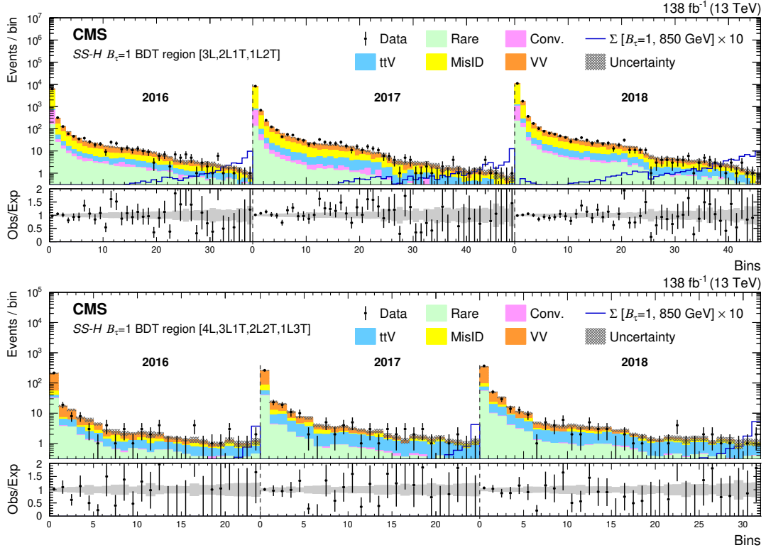
Figure 16: The SS\text{-}H B_\tau = 1 BDT regions for the 3-lepton (upper) and 4-lepton (lower) channels for the 2016–2018 data sets. The lower panel shows the ratio of observed events to the total expected background prediction. The gray band on the ratio represents the sum of statistical and systematic uncertainties in the SM background prediction. The expected SM background distributions and the uncertainties are shown after fitting the data under the background-only hypothesis. For illustration, an example signal hypothesis for the production of the type-III seesaw heavy fermions in the scenario with mixing exclusively to \tau lepton for m_\Sigma = 850 GeV, before the fit, is also overlaid.
