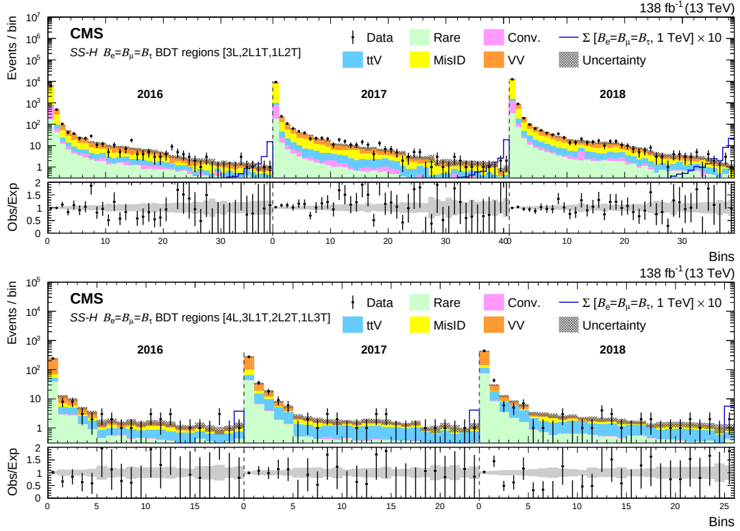
Figure 14: The SS\text{-}H B_e = B_\mu = B_\tau BDT regions for the 3-lepton (upper) and 4-lepton (lower) channels for the 2016–2018 data sets. The lower panel shows the ratio of observed events to the total expected background prediction. The gray band on the ratio represents the sum of statistical and systematic uncertainties in the SM background prediction. The expected SM background distributions and the uncertainties are shown after fitting the data under the background-only hypothesis. For illustration, an example signal hypothesis for the production of the type-III seesaw heavy fermions in the flavor-democratic scenario for m_\Sigma = 1 \text{ TeV} , before the fit, is also overlaid.
