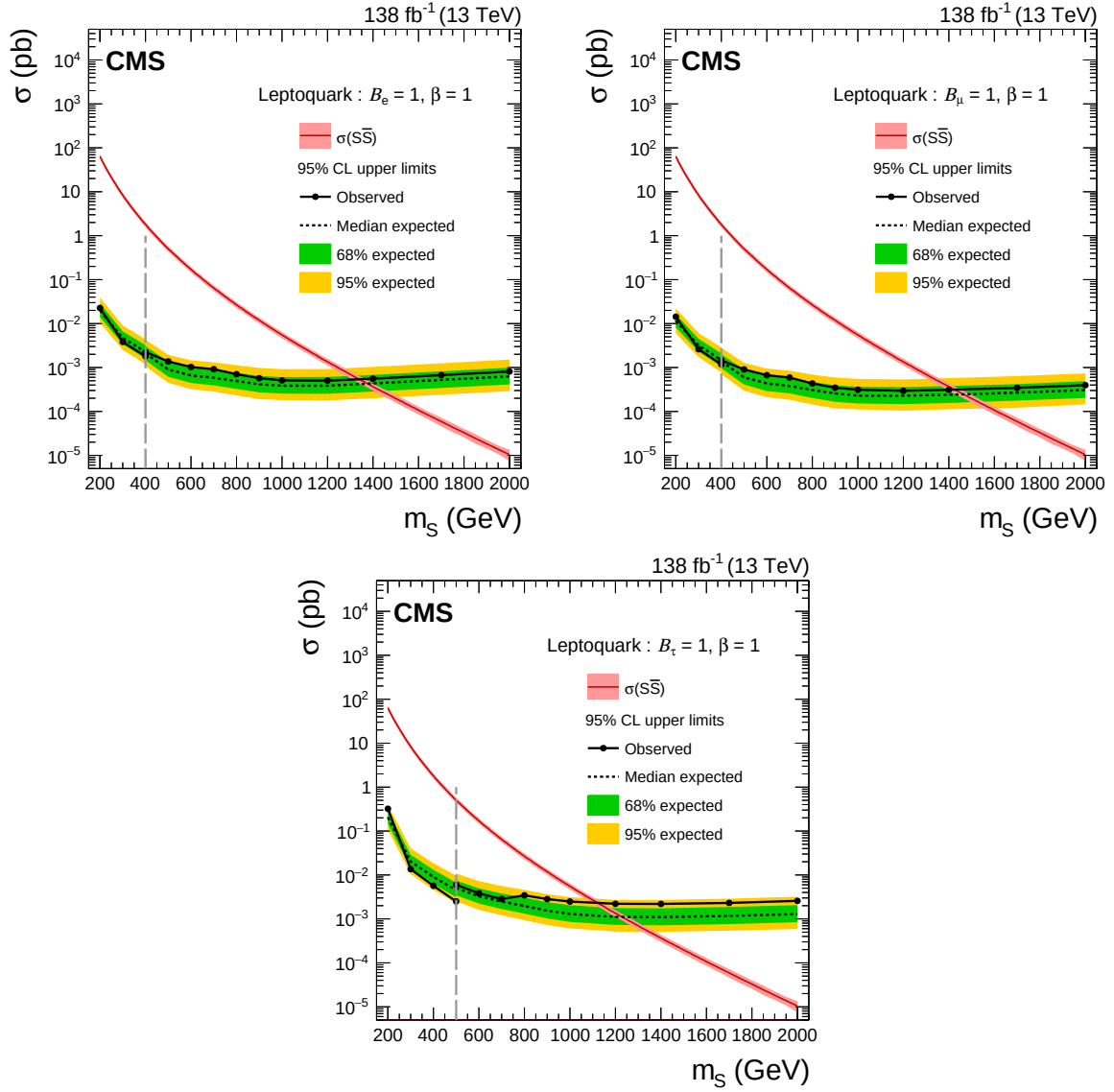
Figure 26: Observed and expected upper limits at 95% CL on the production cross section for the scalar leptokarks: B_e = 1 (upper left), B_\mu = 1 (upper right), and B_\tau = 1 (lower). In each figure, the limits to the left of the vertical dashed gray line are shown from the advanced S_T table, and to the right are shown from the BDT regions.
