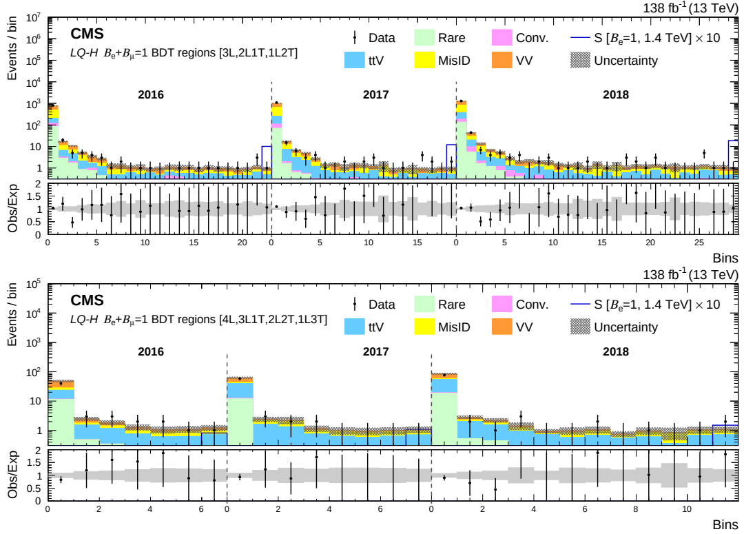
Figure 22: The LQ\text{-}H \mathcal{B}_e + \mathcal{B}_\mu = 1 BDT regions for the 3-lepton (upper) and 4-lepton (lower) channels for the 2016–2018 data sets. The lower panel shows the ratio of observed events to the total expected background prediction. The gray band on the ratio represents the sum of statistical and systematic uncertainties in the SM background prediction. The expected SM background distributions and the uncertainties are shown after fitting the data under the background-only hypothesis. For illustration, an example signal hypothesis for the production of the scalar leptoquark coupled to a top quark and an electron for m_S = 1.4 \text{ TeV} , before the fit, is also overlaid.
