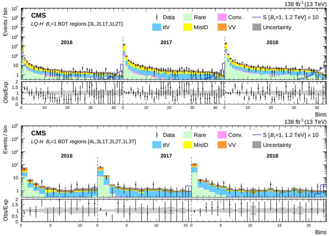
Figure 20: The LQ\text{-}H B_\tau = 1 BDT regions for the 3-lepton (upper) and 4-lepton (lower) channels for the 2016–2018 data sets. The lower panel shows the ratio of observed events to the total expected background prediction. The gray band on the ratio represents the sum of statistical and systematic uncertainties in the SM background prediction. The expected SM background distributions and the uncertainties are shown after fitting the data under the background-only hypothesis. For illustration, an example signal hypothesis for the production of the scalar leptoquark coupled to a top quark and a \tau lepton for m_S = 1.2 \text{ TeV} , before the fit, is also overlaid.
