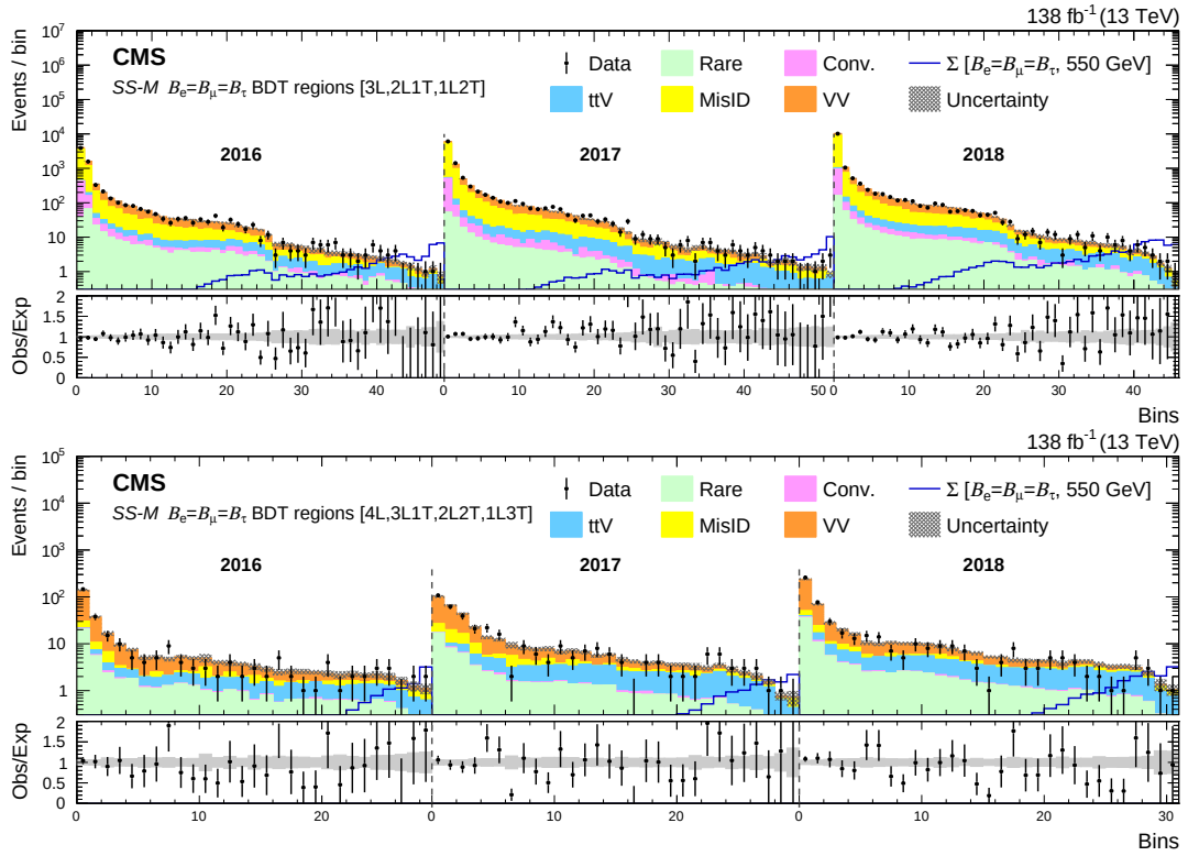
Figure 13: The SS-M B_e = B_\mu = B_\tau BDT regions for the 3-lepton (upper) and 4-lepton (lower) channels for the 2016–2018 data sets. The lower panel shows the ratio of observed events to the total expected background prediction. The gray band on the ratio represents the sum of statistical and systematic uncertainties in the SM background prediction. The expected SM background distributions and the uncertainties are shown after fitting the data under the background-only hypothesis. For illustration, an example signal hypothesis for the production of the type-III seesaw heavy fermions in the flavor-democratic scenario for m_\Sigma = 550 \text{ GeV} , before the fit, is also overlaid.
