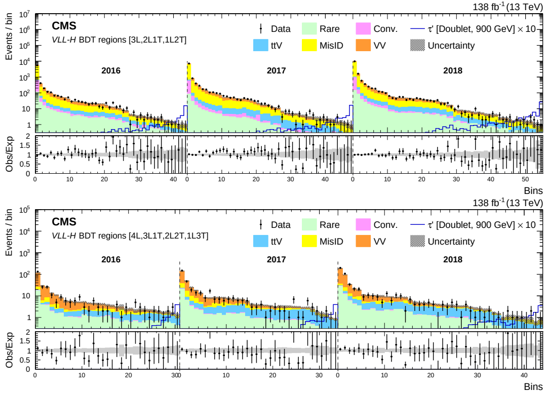
Figure 18: The VLL-H BDT regions for the 3-lepton (upper) and 4-lepton (lower) channels for the 2016–2018 data sets. The lower panel shows the ratio of observed events to the total expected background prediction. The gray band on the ratio represents the sum of statistical and systematic uncertainties in the SM background prediction. The expected SM background distributions and the uncertainties are shown after fitting the data under the background-only hypothesis. For illustration, an example signal hypothesis for the production of the vector-like \tau lepton in the doublet scenario for m_{\tau'} = 900 GeV, before the fit, is also overlaid.
