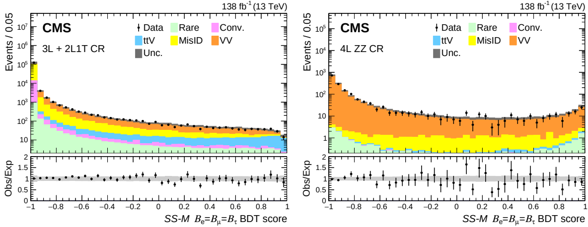
Figure 6: Distributions of BDT score from the SS\text{-}M B_e = B_\mu = B_\tau BDT are shown for the 3L+2L1T CR (left), and the 4L ZZ CR (right). The 3L+2L1T CR consists of the 3L OnZ, 3L Z\gamma , and 2L1T MisID CRs. The lower panel shows the ratio of observed events to the total expected background prediction. The gray band on the ratio represents the sum of statistical and systematic uncertainties in the SM background prediction.
