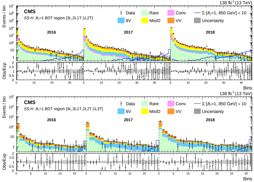
Figure 16: The SS-H B_\tau = 1 BDT regions for the 3-lepton (upper) and 4-lepton (lower) channels for the 2016–2018 data sets. The lower panel shows the ratio of observed events to the total expected background prediction. The gray band on the ratio represents the sum of statistical and systematic uncertainties in the SM background prediction. The expected SM background distributions and the uncertainties are shown after fitting the data under the background-only hypothesis. For illustration, an example signal hypothesis for the production of the type-III seesaw heavy fermions in the scenario with mixing exclusively to \tau lepton for m_\Sigma = 850 \text{ GeV} , before the fit, is also overlaid.
