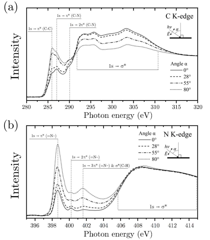
Figure 3: The (a) carbon and (b) nitrogen NEXAFS spectra of dye-modified graphene recorded along with variation relative to the sample surface plane of the electric field vector incidence angle of linearly polarized X-ray radiation. The angle \alpha determines the orientation of the X-ray beam relative to the normal of the sample. The angle of 0^\circ corresponds to the case when the electric field vector is parallel to the sample surface; the angle of 90^\circ means that the electric field vector is perpendicular to it.
