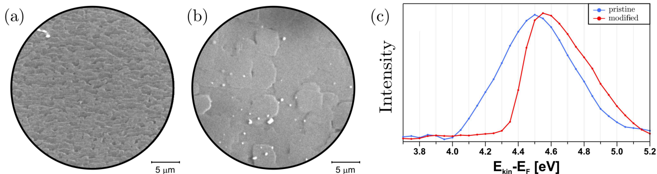
Figure 7: UV-PEEM images of graphene grown on \beta -SiC(001) before (a) and after chemical modification by the Neutral Red organic dye using the diazonium chemistry approach. (c) Secondary electron cutoff, which represents the work function change as a result of the chemical modification of graphene/SiC(001).
