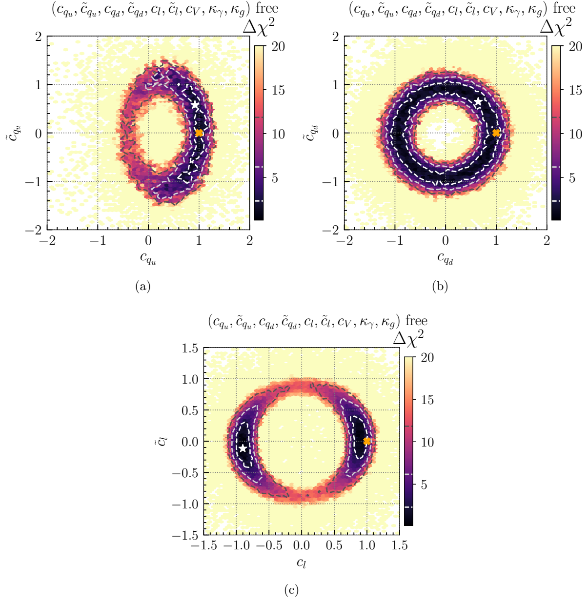
Figure 18: Results of fits to the LHC measurements in the (a) (c_{qu}, \tilde{c}_{qu}) , (b) (c_{qd}, \tilde{c}_{qd}) , and (c) (c_l, \tilde{c}_l) parameter plane. All parameters listed above the plot panels are floated freely. The legend corresponds to the one in Fig. 2.
