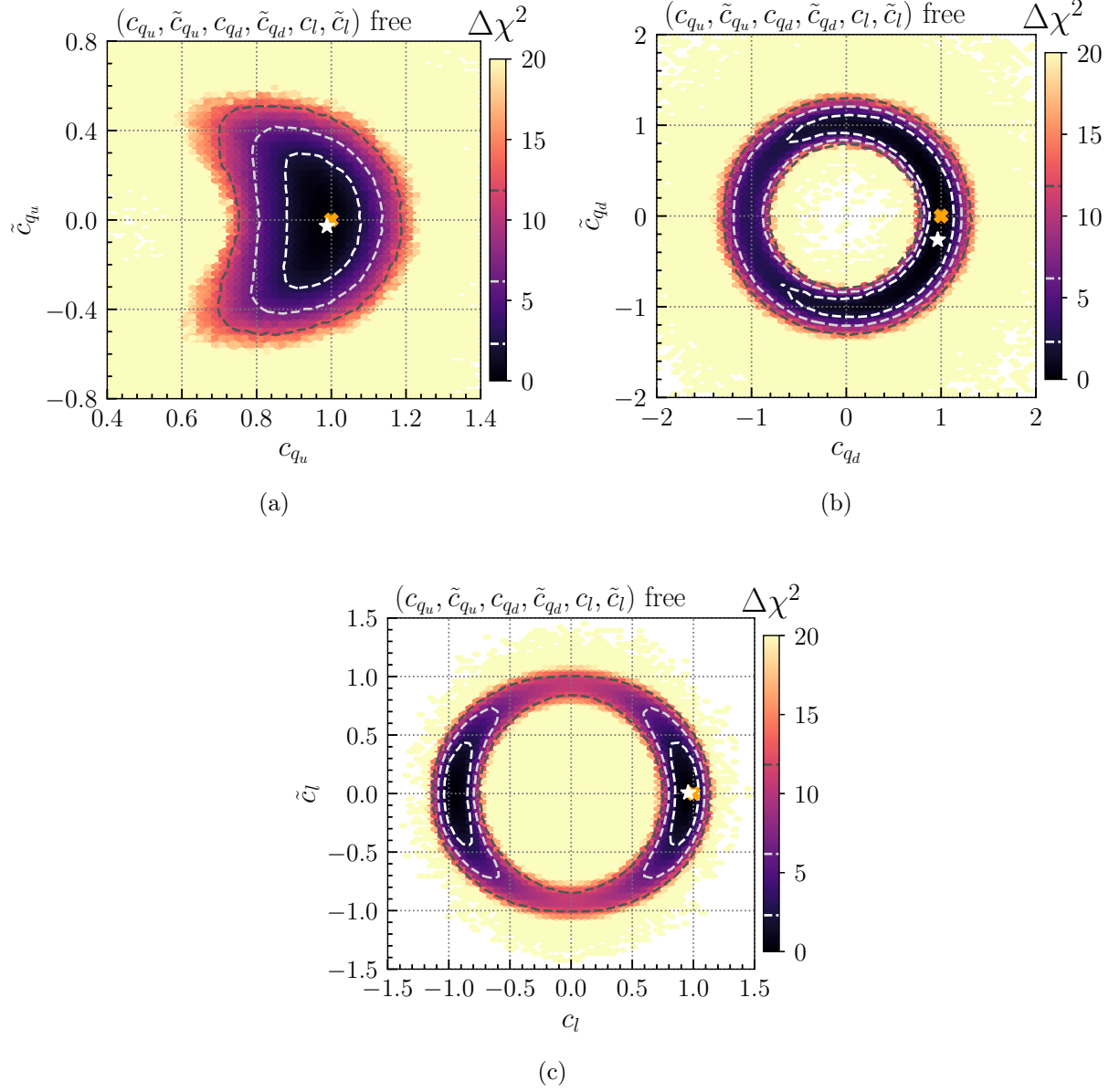
Figure 16: Results of fits to the LHC measurements in the (a) (c_{qu}, \tilde{c}_{qu}) , (b) (c_{qd}, \tilde{c}_{qd}) , and (c) (c_l, \tilde{c}_l) parameter plane. For each plot the indicated coupling modifiers are free-floating while all the other parameters are set to their SM values. The legend corresponds to the one in Fig. 2.
