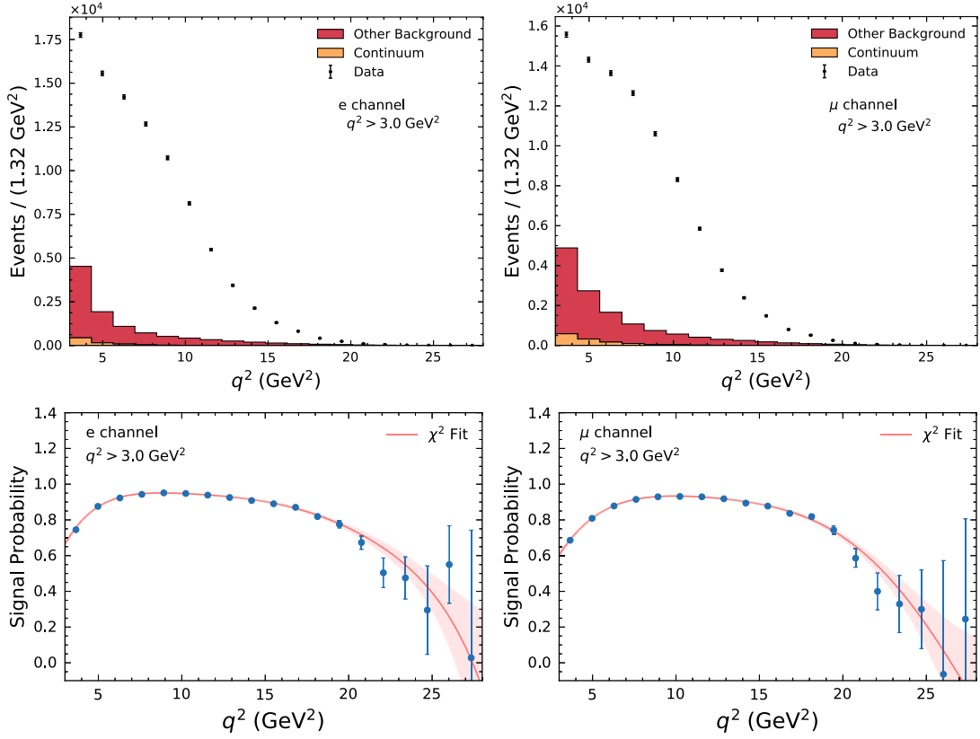
FIG. 4. The reconstructed q^2 distributions with an example q^2 threshold selection of 3.0 GeV 2 (top) for electron (left) and muon (right) candidates and the determined binned signal probabilities (bottom) are shown. The background contributions are scaled to their estimated values using the fit described in the text. The binned signal probabilities are obtained by a fit of a polynomial of a given order n (red curve).
