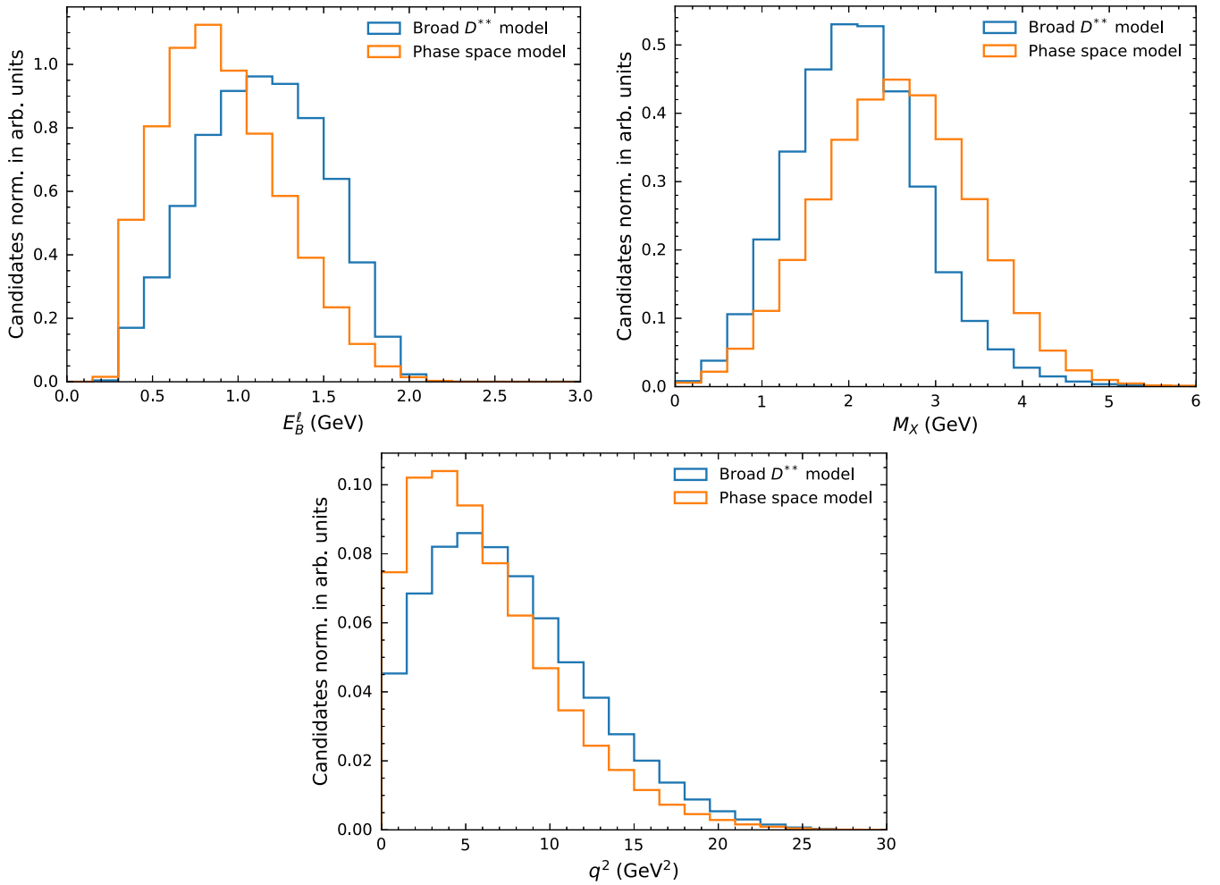
FIG. 9. Comparisons between the different B \rightarrow D_{\text{gap}}^{**} \ell \bar{\nu}_\ell decay models for the reconstructed lepton energy in the signal B rest frame E_\ell^B (upper left), the M_X (upper right), and the q^2 (bottom) distributions.
