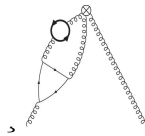
Figure 3. 2-mass 3-loop diagram.
