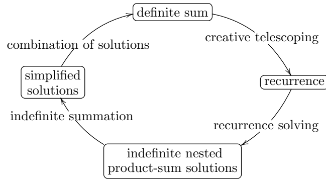
Figure 2. Sigma's summation spiral; see [167].
