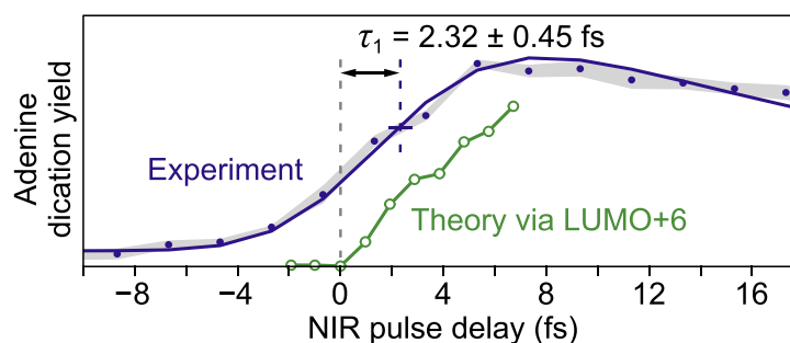
Figure 3. Delayed production of stable adenine dications. Zoom-in on the central part of a XUV-pump–NIR-probe scan [6], with experimental data points as filled circles and the fitted curve showing a significantly delayed onset (see methods section for the definition of \tau_1 ) in the enhancement of the dication yield. The grey shaded areas show \pm one standard error of the mean of seven successive scans in alternating directions. Open circles show the main part of the theoretical result, calculated using the non-equilibrium Green's function method. The theoretical signal remains zero when the pulses fully overlap and only starts to increase at positive delays, because shake-up to the selected LUMO+6 state takes time. The result via other states does not show such a strong and late increase [6, supplementary figure S18].
