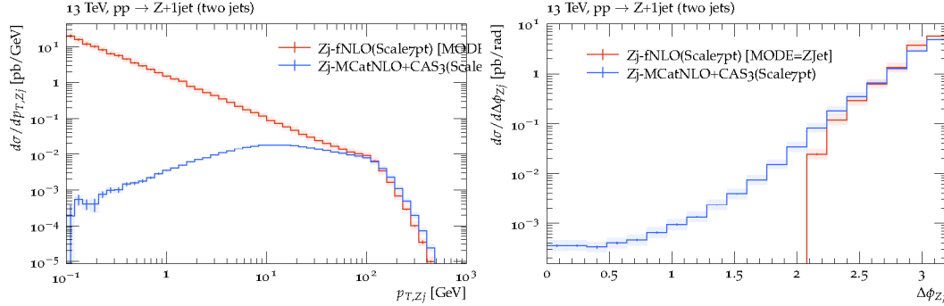
Figure 1: Transverse momentum spectrum of the Z+jet-system p_{T,Zj} (left) and \Delta\phi_{Zj} distribution (right). The predictions are shown for fixed NLO (MCatNLO(fNLO) and after inclusion of PB-TMDs (MCatNLO+CAS3).
