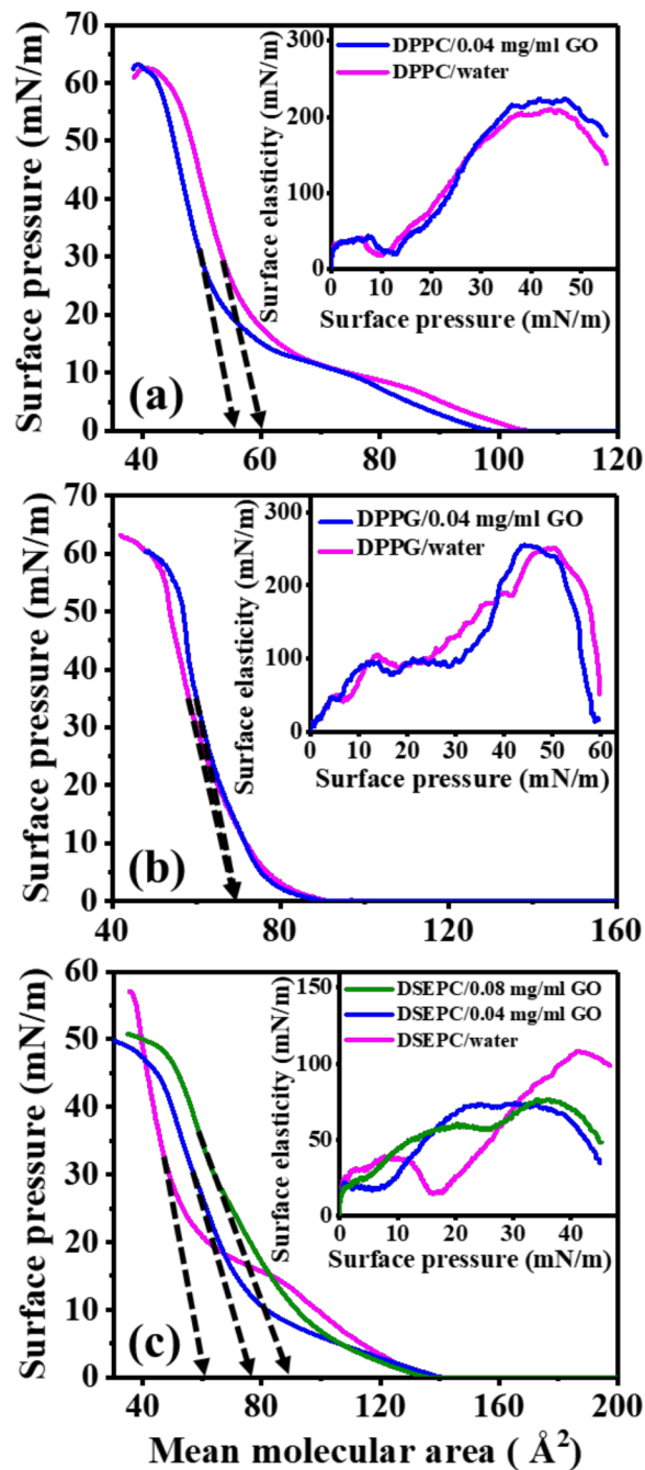
Figure 1. Surface pressure-area isotherms of lipid monolayers at air-water and air-GO aqueous interface. Isotherms of (a) neutrally charged DPPC, (b) negatively charged DPPG and (c) positively charged DSEPC. The intercepts of dashed lines with abscissa signify the limiting molecular area of a lipid in liquid condensed phase. Inset: Variation of in-plane elasticity or surface compressional modulus of lipid monolayers as a function of surface pressure. The GO aqueous dispersion of two different concentrations, namely, 0.04 mg/ml and 0.08 mg/ml have been used as the subphase. All measurements were performed at \sim 22^\circ\text{C} .
