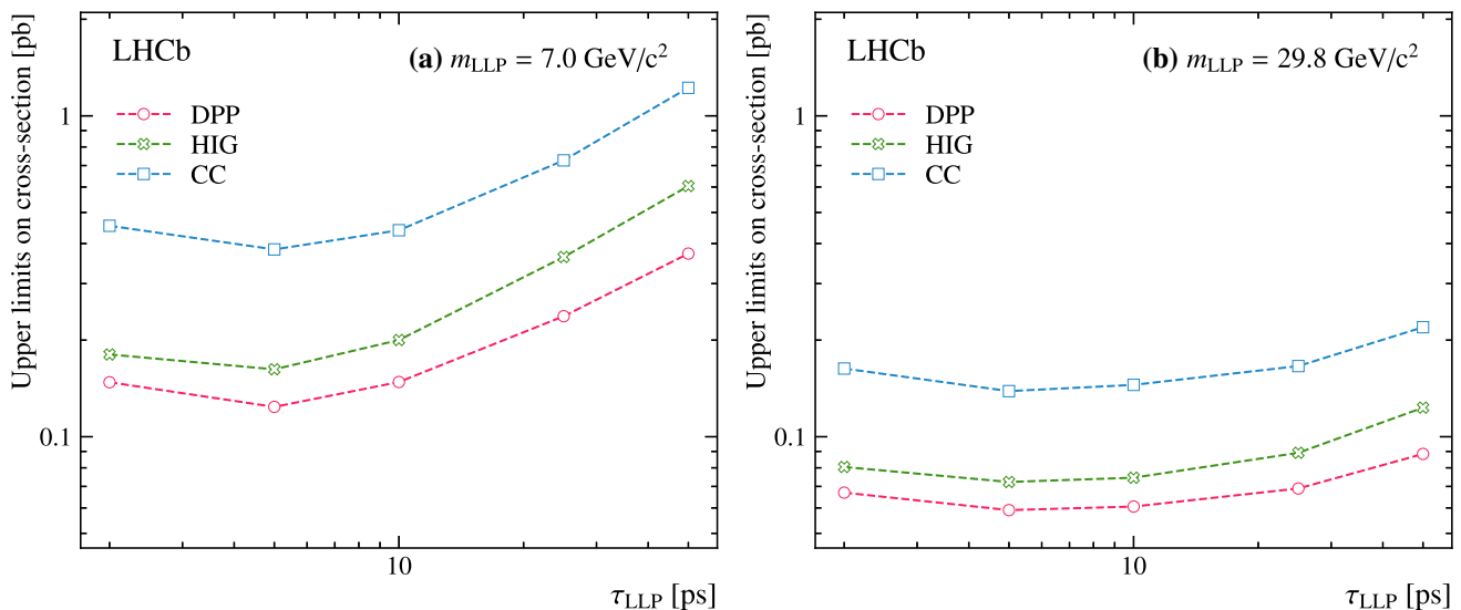
Fig. 7 Observed upper limits on the production cross-sections times branching fraction for a m_{\text{LLP}} = 7 GeV/c 2 and b m_{\text{LLP}} = 29.8 GeV/c 2 as a function of \tau_{\text{LLP}} for the DPP, HIG and CC production mechanisms
