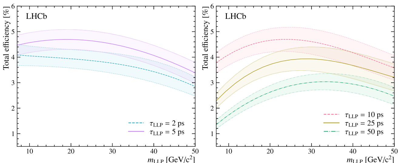
Fig. 5 Total detection efficiency for LLP produced through the DPP mechanism as a function of m_{\text{LLP}} (central line) and its uncertainty (coloured band), obtained for different values of \tau_{\text{LLP}}
