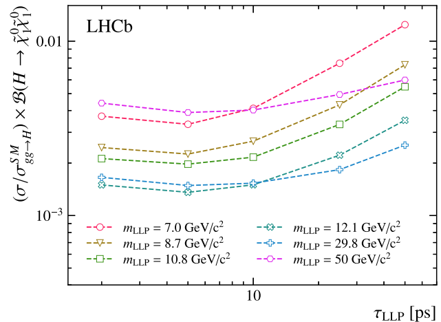
Fig. 8 Observed limits on the (\sigma/\sigma_{\text{gg} \rightarrow H}^{\text{SM}}) \times \mathcal{B}(H^0 \rightarrow \tilde{\chi}_1^0 \tilde{\chi}_1^0) , assuming \mathcal{B}(\tilde{\chi}_1^0 \rightarrow e^\pm \mu^\mp \nu) = 1 as a function of \tau_{\text{LLP}} for different m_{\text{LLP}} values. The value of the gluon-gluon fusion production cross-section used is 48.6 \pm 3.5 pb [47]
