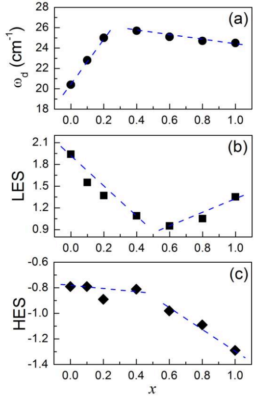
Fig. 4. (a) Crossover frequency \omega_d (\equiv \omega_{\text{bos}}) , and (b) low-energy slope (LES) and (c) high-energy slope (HES) of the boson peak (BP) for the investigated glasses in the (\text{As}_2\text{S}_3)_x(\text{GeS}_2)_{1-x} system as a function of composition x . The dashed lines are drawn as a guide for the eye.
