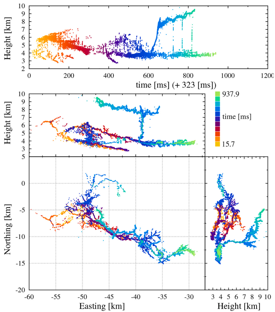
Fig. A.6. Overview of Flash A. The weather map for the time of this flash can be retrieved from ( KNMI, 2018 ).
