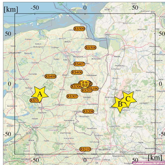
Fig. A.5. Layout of the Dutch LOFAR stations. The core of LOFAR is indicated by the yellow \oplus sign while the yellow stars show the general location of flashes A, B, and C that are discussed in this work. The black frame indicates the general area ( 140 \times 140 \text{ km}^2 ) where flashes can be mapped accurately. (For interpretation of the references to colour in this figure legend, the reader is referred to the web version of this article.)
