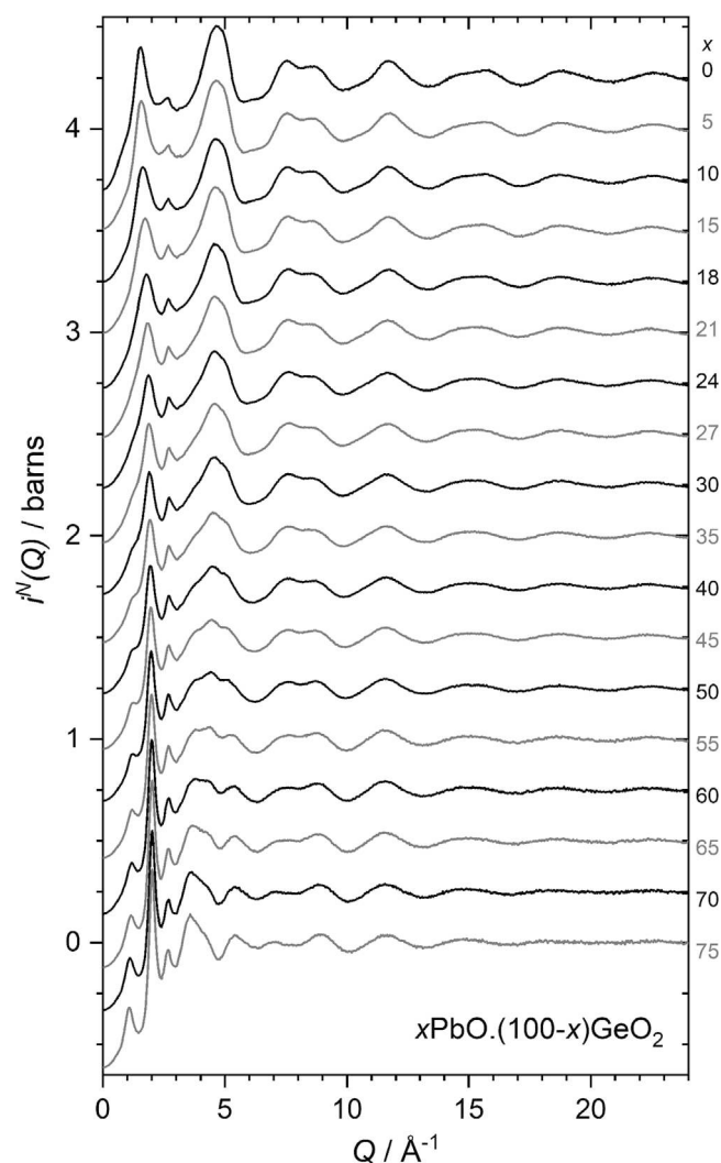
FIGURE 5 Neutron distinct scattering from lead germanate glasses, compared to that for vitreous germania. Molar compositions (nominal) are indicated and vertical offsets have been used for clarity
