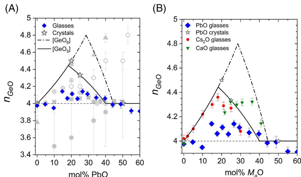
FIGURE 1 Ge–O coordination numbers as a function of PbO–GeO 2 glass composition, using neutron diffraction in this study (blue diamonds), extracted by means of integration of rT^N(r) (Table 4). Comparison is made in (A) to values reported in the literature using neutron diffraction 21 (triangles), Ge K-edge EXAFS (circles: filled, 11 open, 14 with crosses 15 ) and classical molecular dynamics 17 (squares). Values for crystalline lead germanates 56,57,67,74,75 are also shown (open stars). Curves are the analytical models of Hannon et al. 59 for five (solid) or six (dash-dot) coordinated germanium. In (B) comparison is made to Ge–O coordination numbers from neutron diffraction for vitreous calcium 53 and caesium 55 germanates. In colour online
