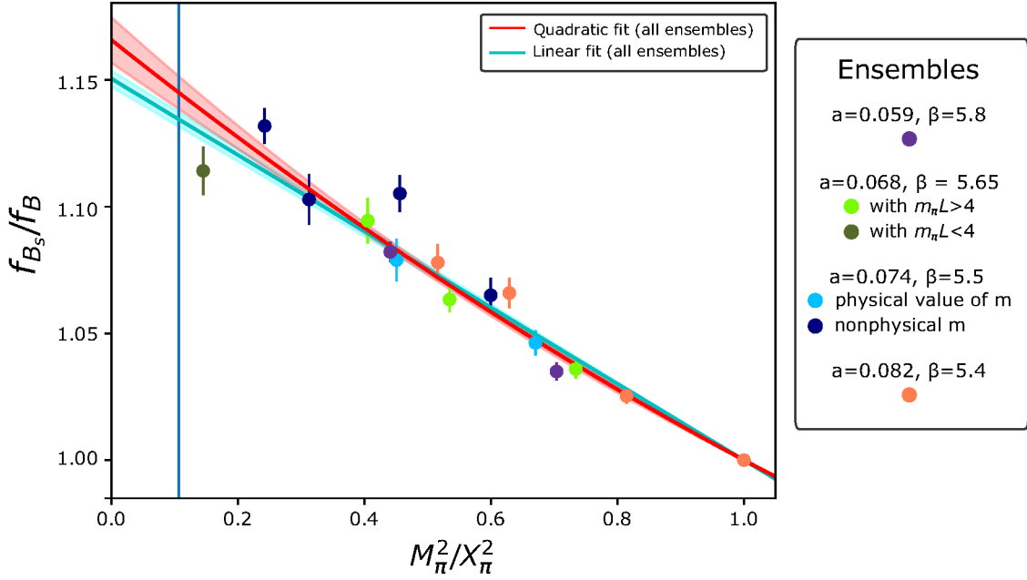
Figure 2: f_{B_s}/f_B for a variety of lattice ensembles. The linear and quadratic fits shown are for all ensembles, and are constrained to pass through the fixed point (1,1).
